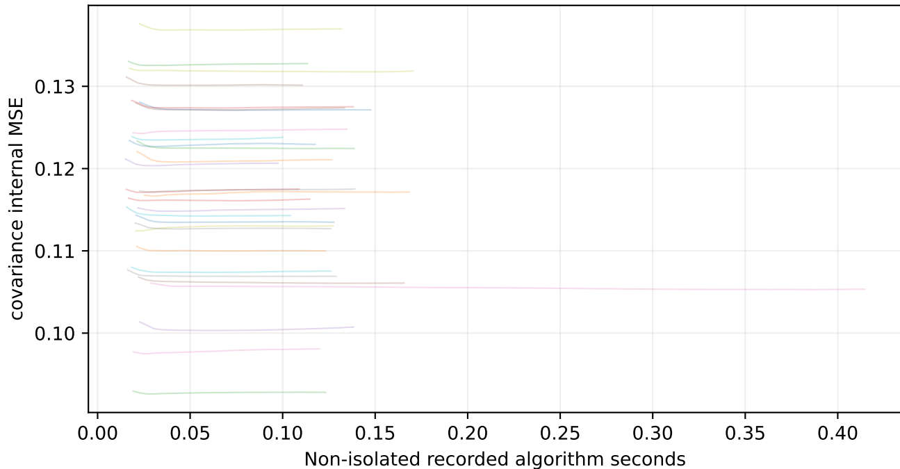
ex1_arff_historical_corrected_covariance — 30 recorded histories
