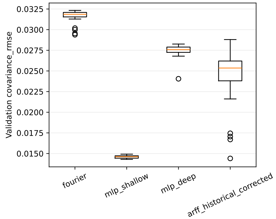
ex1 —30 seeds, resolved production
