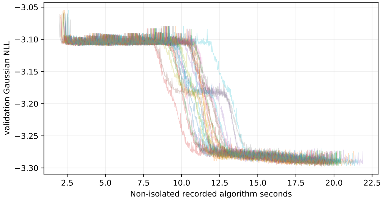
ex1_fourier — 30 recorded histories
