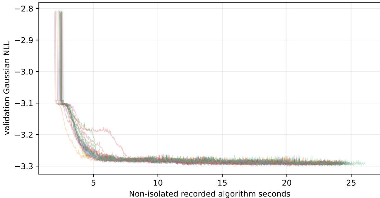
ex1_mlp_deep — 30 recorded histories
