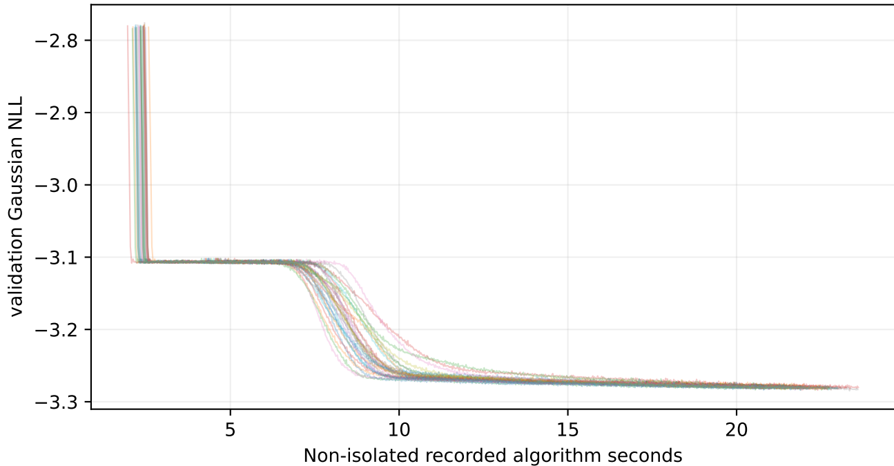
ex1_mlp_shallow — 30 recorded histories
