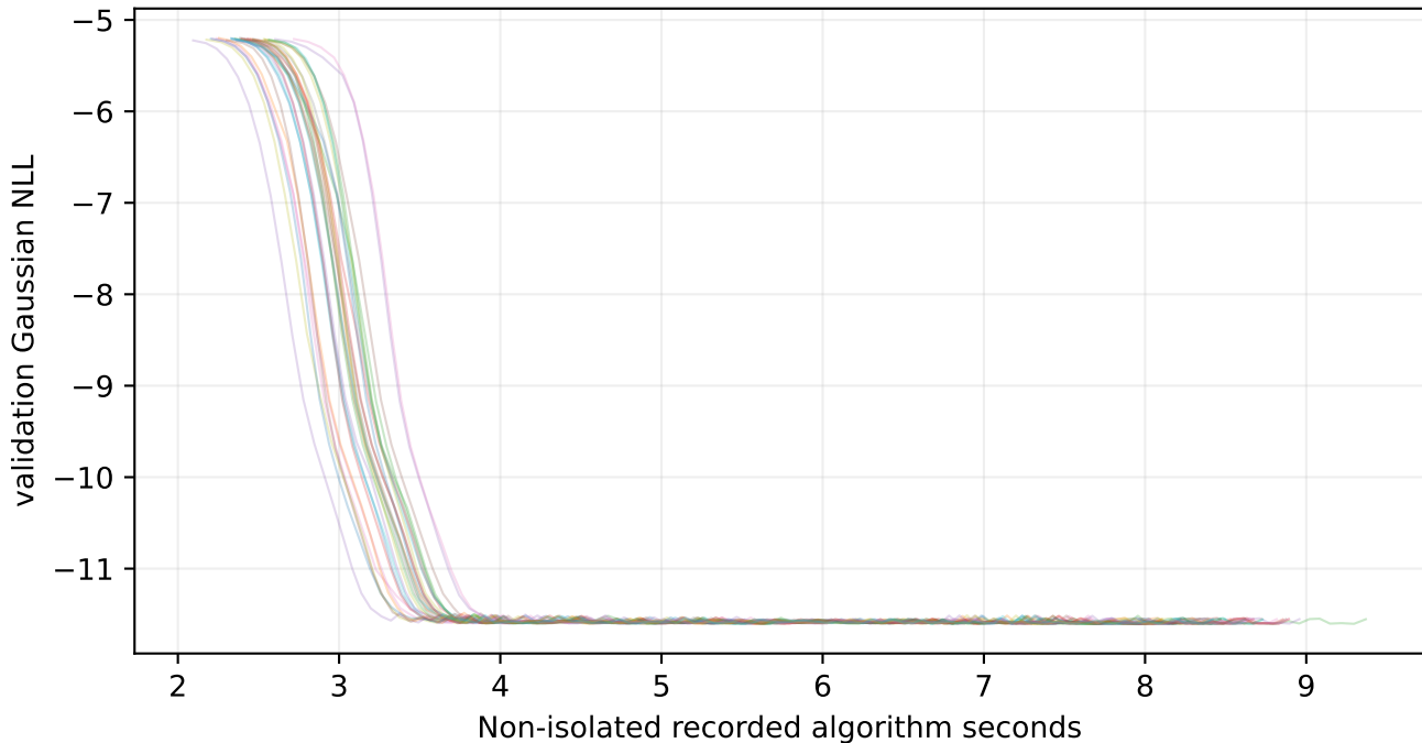
ex2_mlp_deep —30 recorded histories
