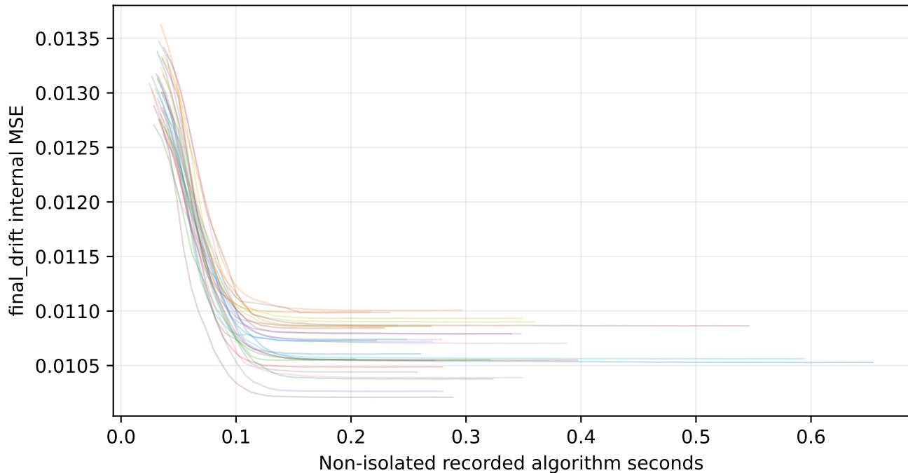
ex5_arff_historical_corrected_final_drift —30 recorded histories
