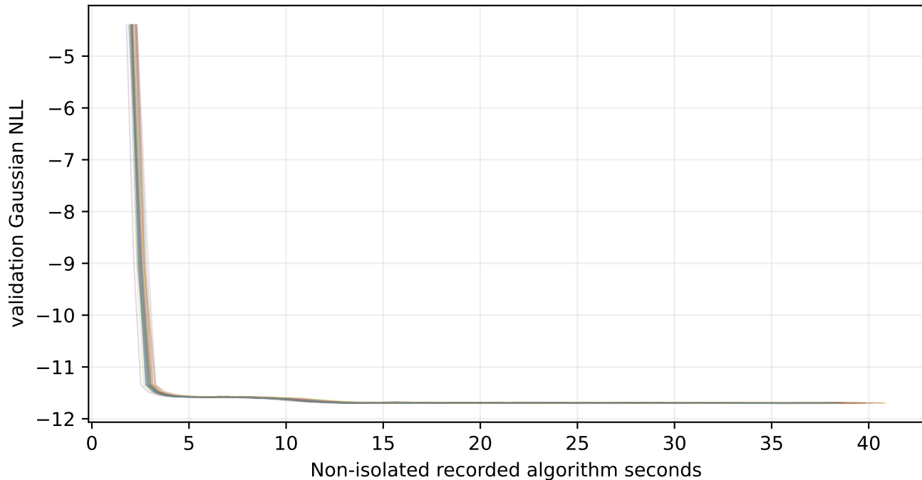
ex5_mlp_shallow —30 recorded histories
