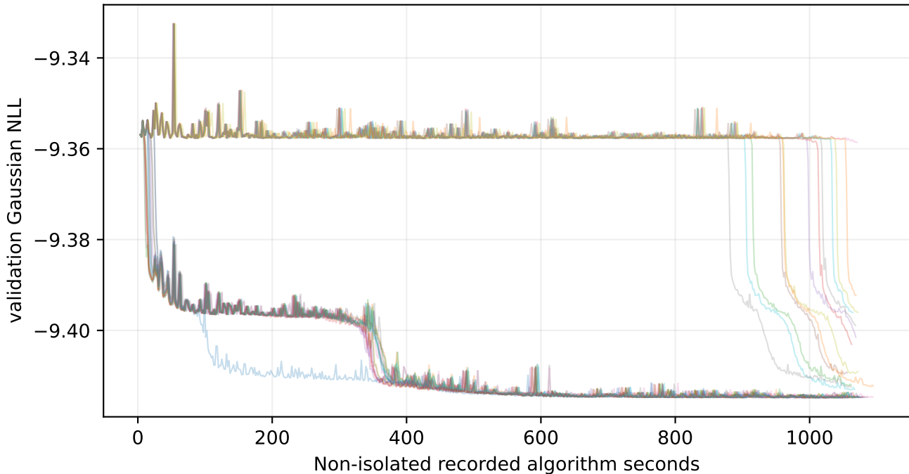
ex6_mlp_shallow — 30 recorded histories
