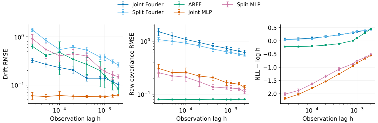
Figure 5: Ex8 test sensitivity to lag at N = 640000, K = 1024 , mean \pm sample SD over ten fitting seeds. \text{NLL} - \log h removes the two-dimensional density-scale term, not transition-shape differences. The .002 endpoint satisfies the pre-existing oracle bias tolerance, not a fitted optimum.
