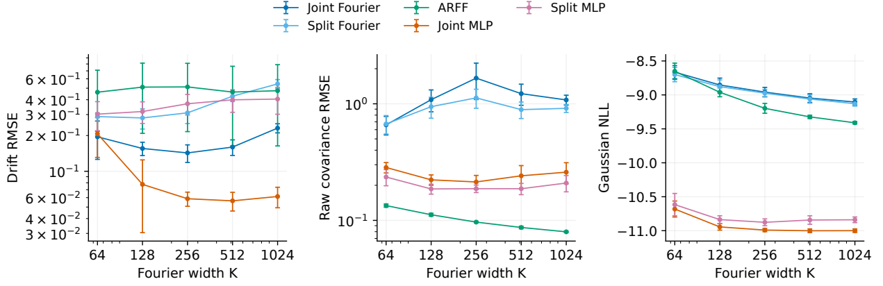
Figure 6: Descriptive Ex8 test performance versus Fourier width K at fixed N = 640000 , h = 10^{-4} , ten seeds. K = 64, 128, 256, 512, 1024 gives Fourier parameter counts 896,1792,3584,7168,14336; matched two-layer MLP widths 18,27,39,57,81 give counts 887,1814,3554,7244,14180. No asymptotic rate is asserted.
