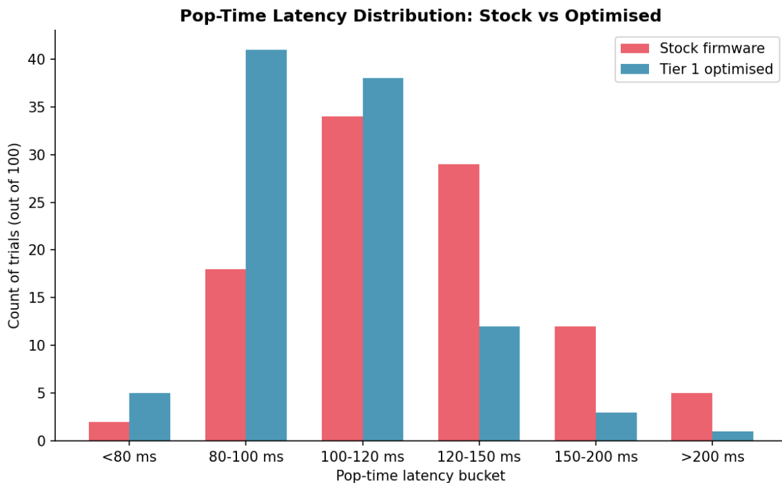
Figure 3. Latency distribution shift between stock and optimised firmware across 100 benchmark trials.
