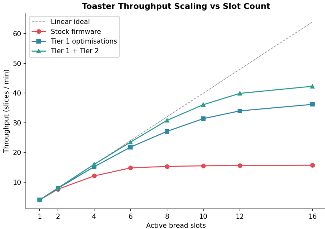
Figure 2. Throughput scaling with the number of active bread slots, showing how the Tier 1 optimisations extend the linear regime.
