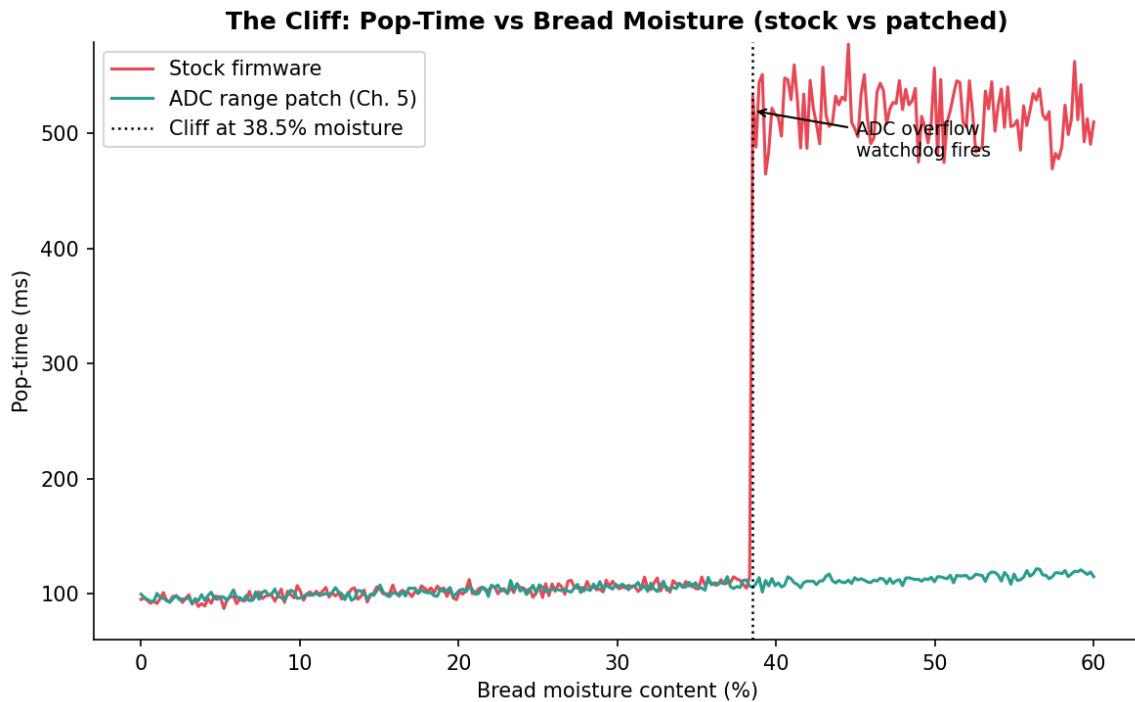
Figure 4. The performance cliff at 38.5% bread moisture: pop-time jumps from approximately 100 ms to 520 ms due to ADC overflow in the thermal probe path.
