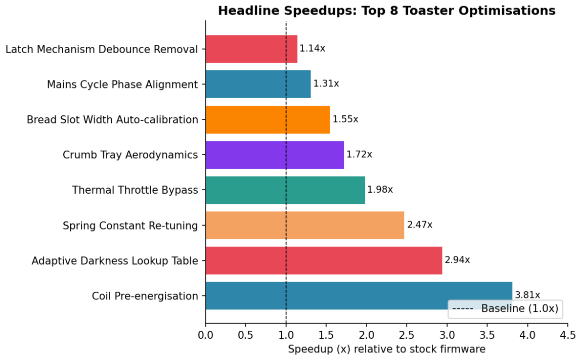
Figure 1. Headline speedup summary: geometric mean over all bread types per optimisation.
