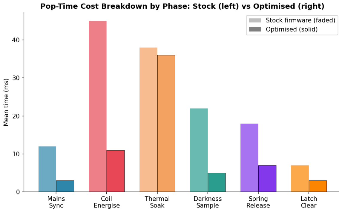
Figure 6. Per-phase cost breakdown: stock firmware vs optimised. Left bar per phase is stock; right bar is optimised.
