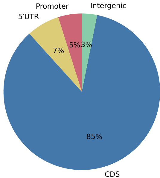
GCCGGC m4C sites (n=1659)
