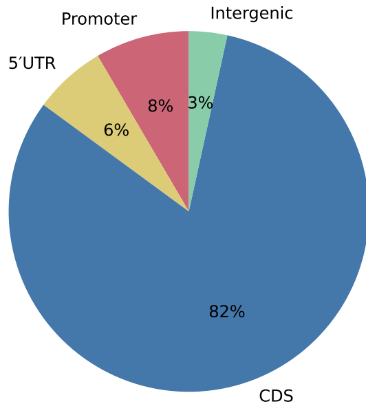
AAGCCCG m4C sites (n=1078)
