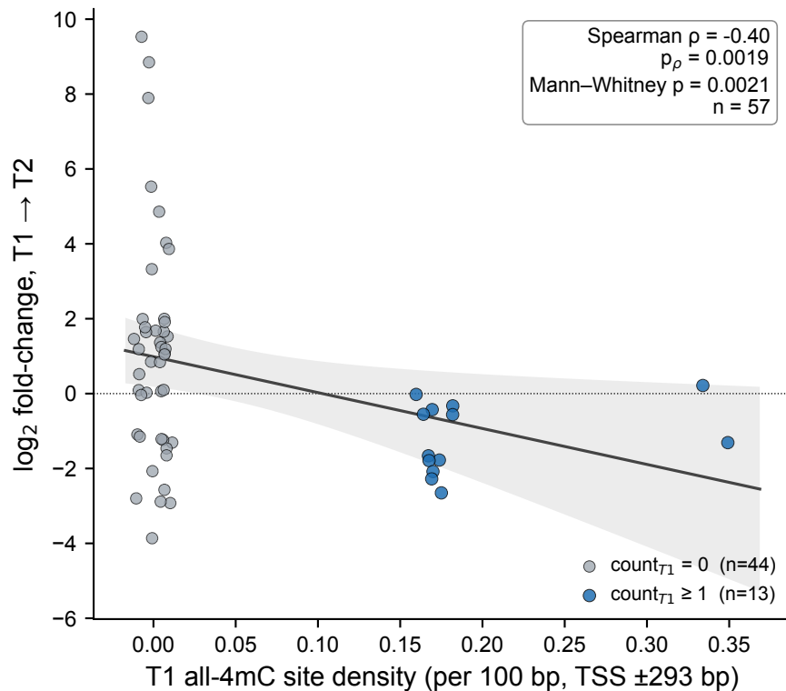
(a) Exposed TFs
