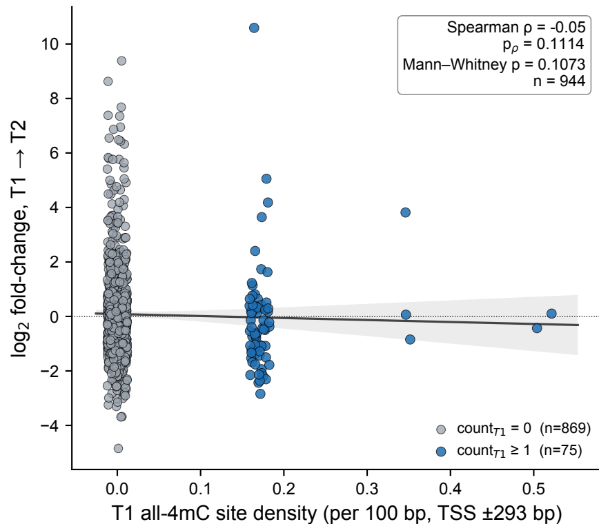
(b) Shielded TFs (control)
