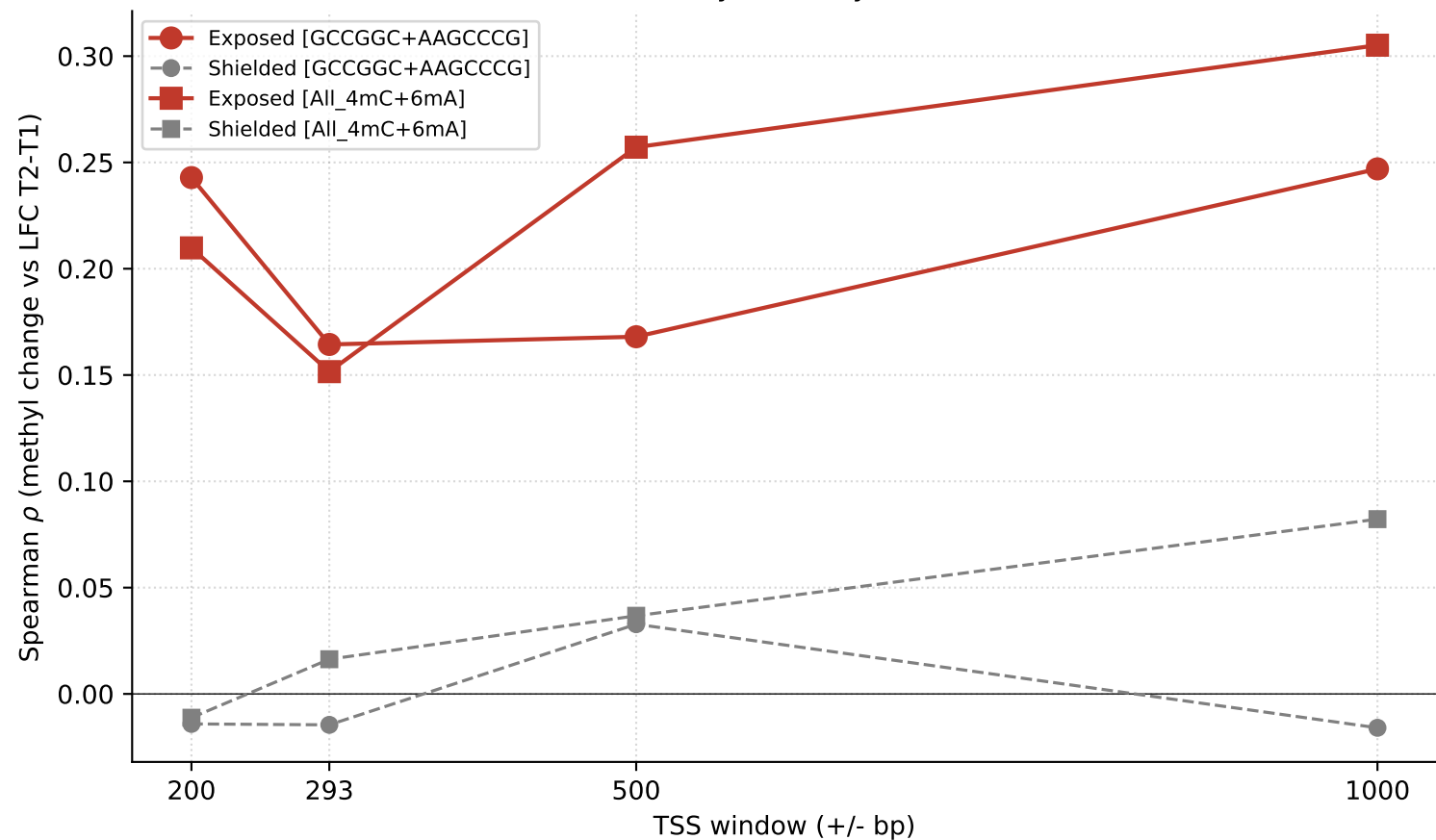
Window sensitivity of methyl-LFC correlation
