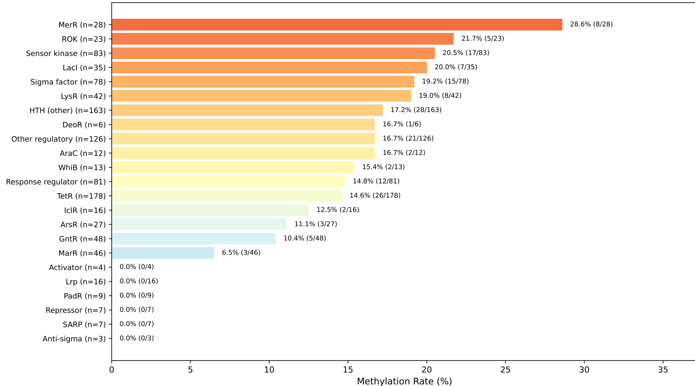
Methylation Rate by TF Family (families with n &gt;= 3 genes)
