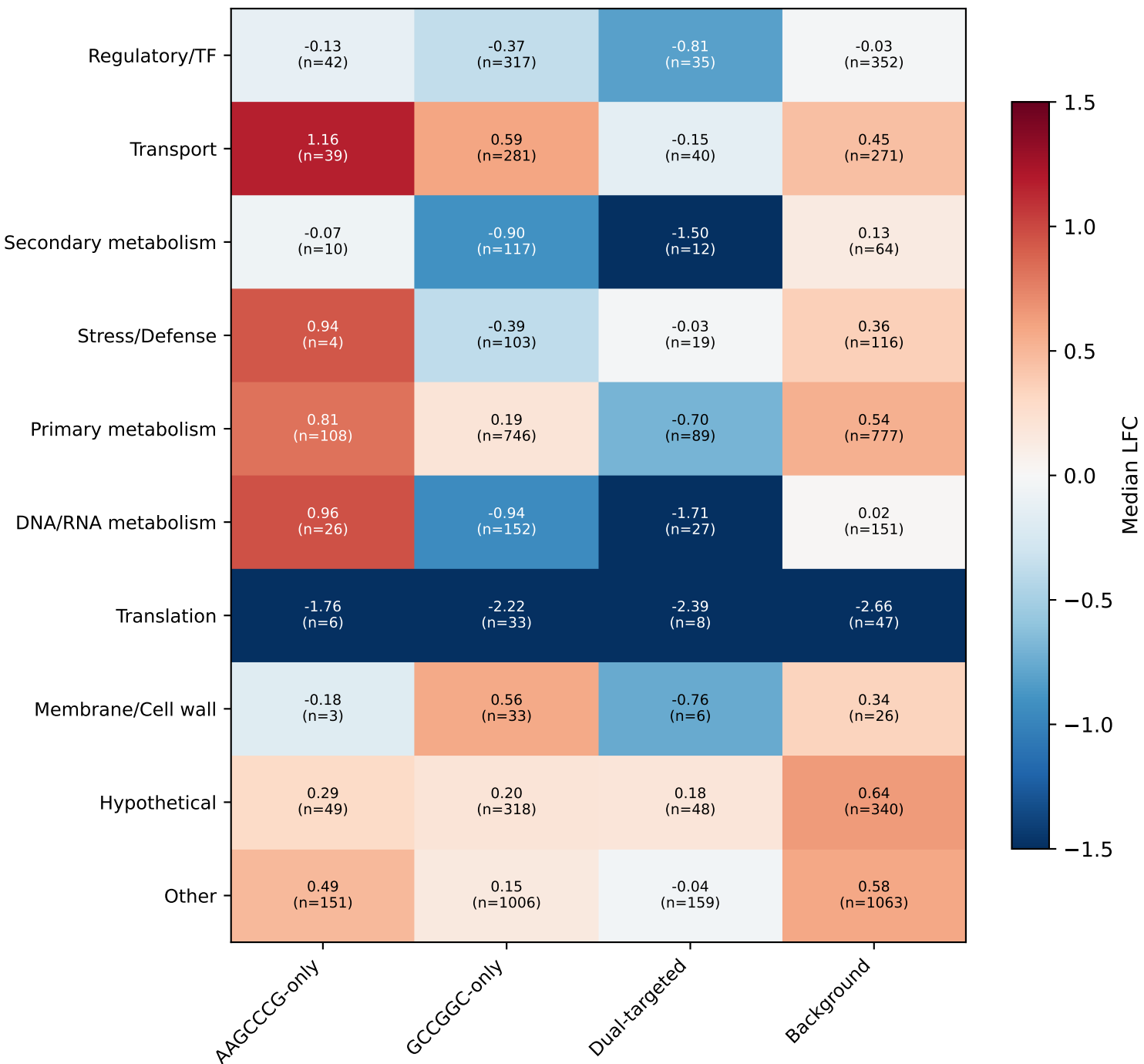
Median LFC T3vsT1
