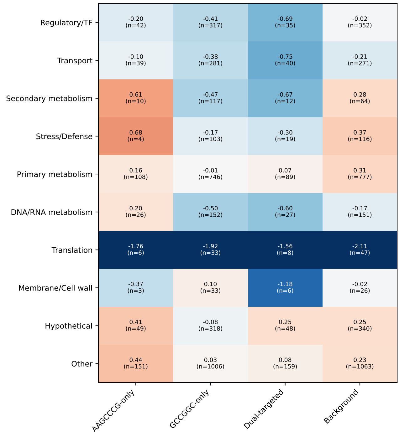
Median LFC T2vsT1
