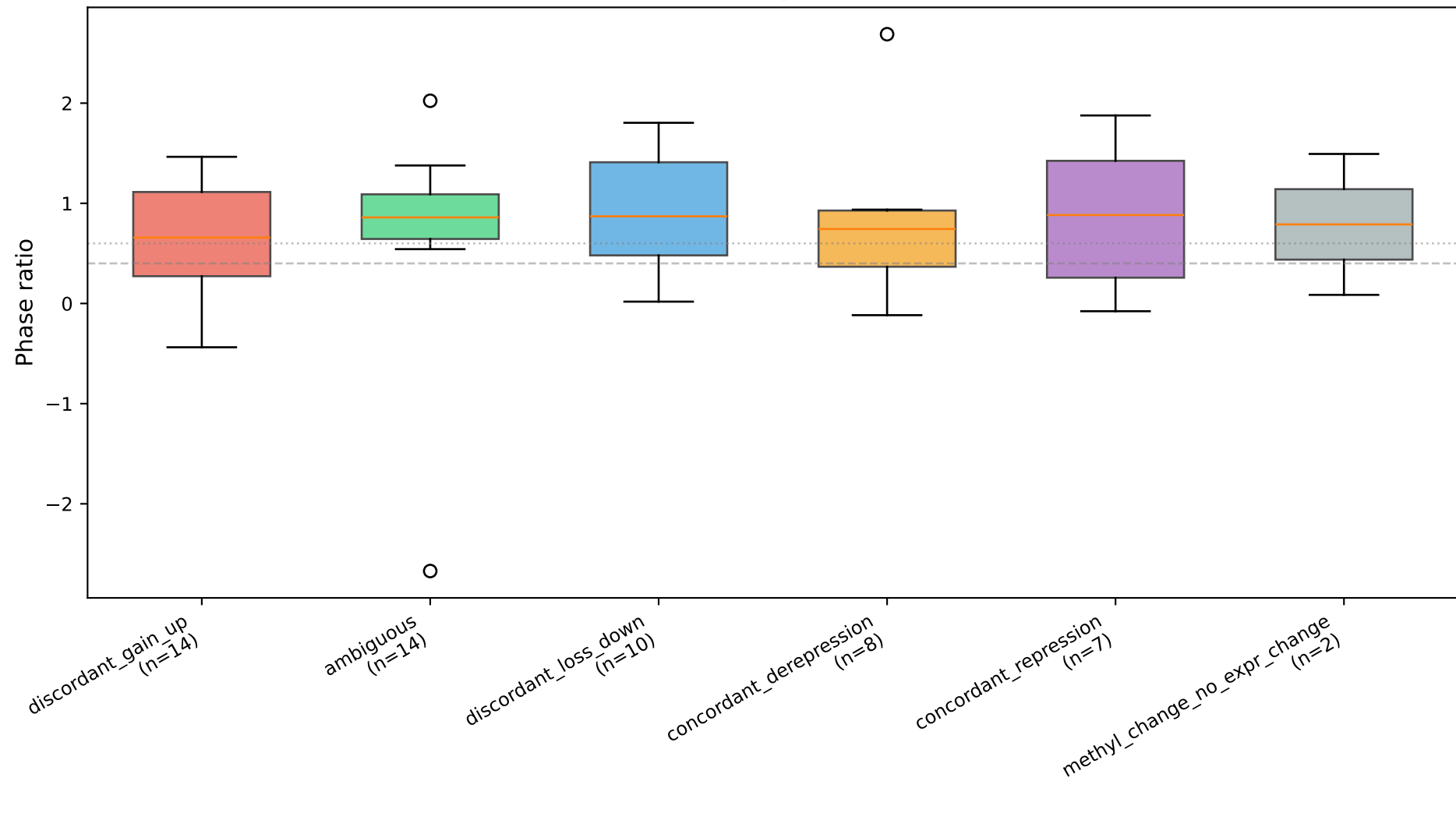
H34: Phase ratio by coordination type (T3) (Kruskal-Wallis p=7.580e-01 )
