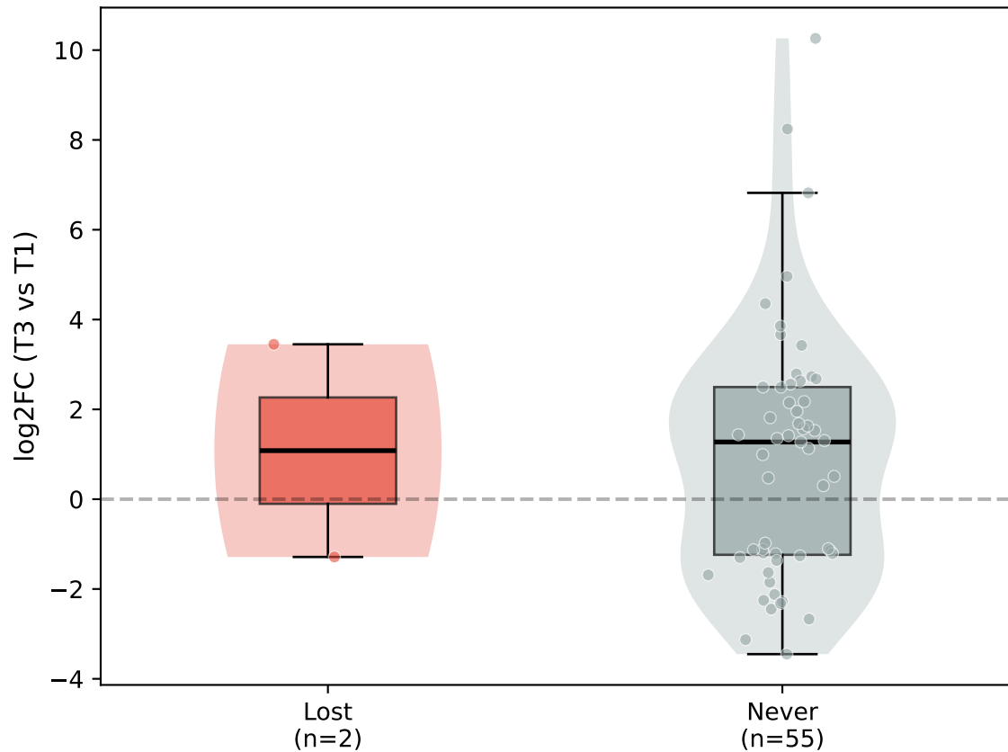
B) LFC distribution by AAGCCCCG status (T3 vs T1, Exposed TFs only)
