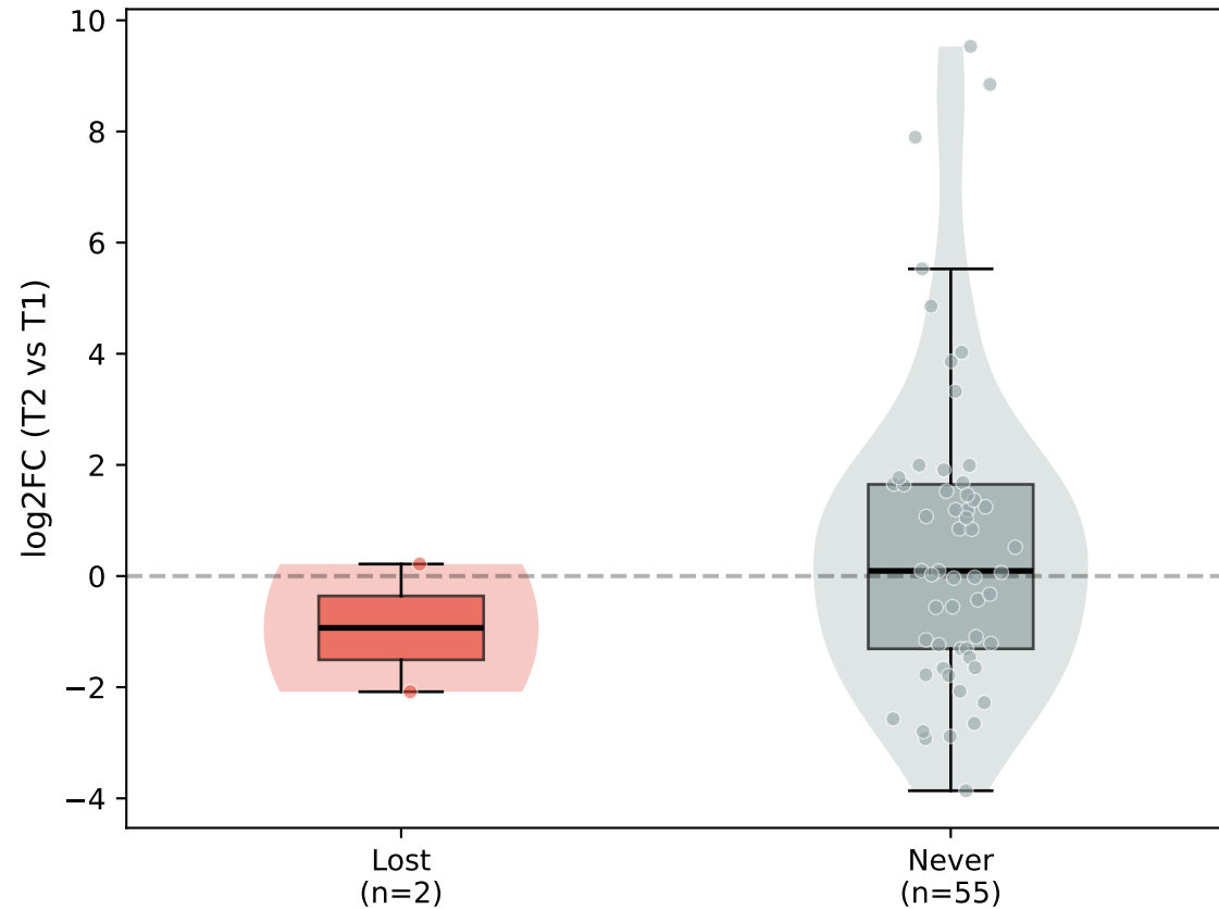
A) LFC distribution by AAGCCCCG status (Exposed TFs only)
