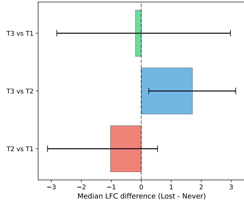
C) Effect size by transition (with 95% bootstrap CI)
