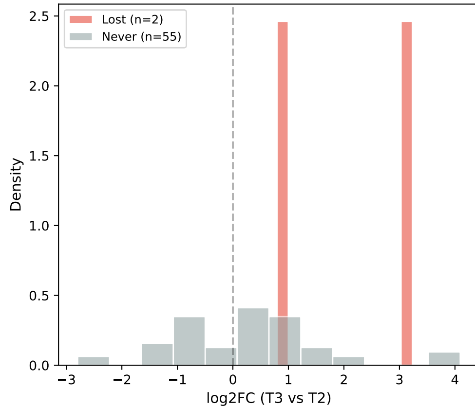
B) T2→T3 (after MTase drop) p=1.80e-01
