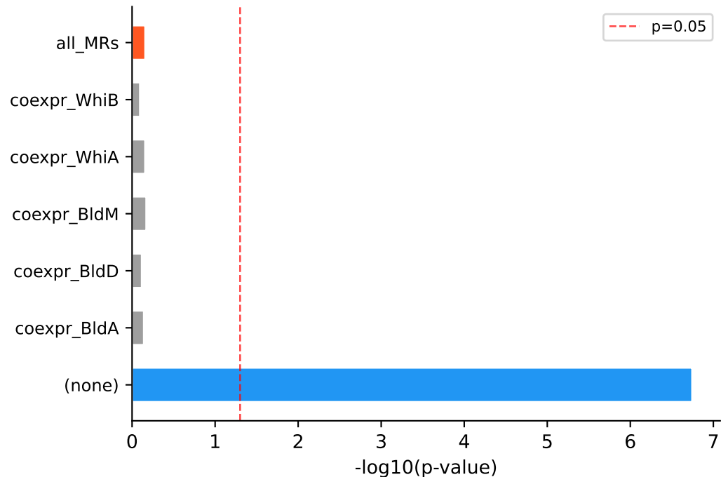
Significance
