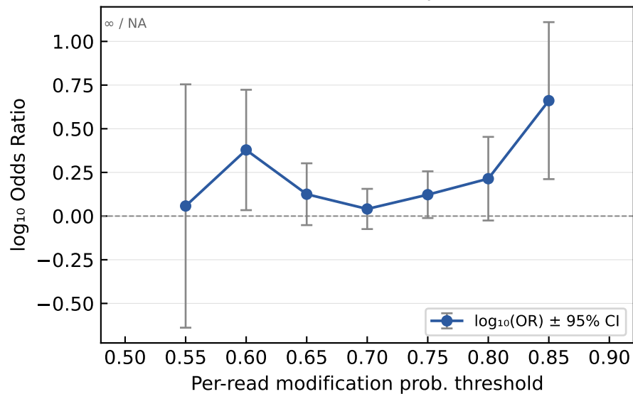
Site-level OR (freq ≥ 0.5)
