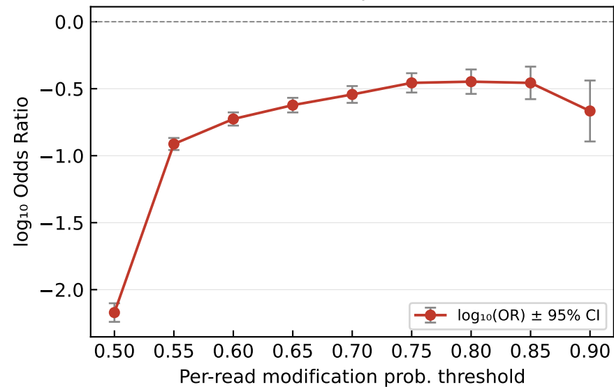
Per-read pair OR
