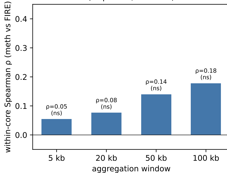
(b) No within-compartment resolution (all p > 0.1 , 5–100 kb)
