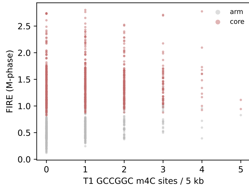
(a) Genome-wide co-localisation Spearman \rho = 0.32 (= core/arm contrast)
