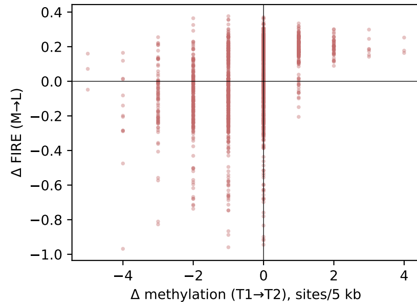
(c) Developmental co-change Spearman \rho = 0.43 ( p = 1e-77 )
