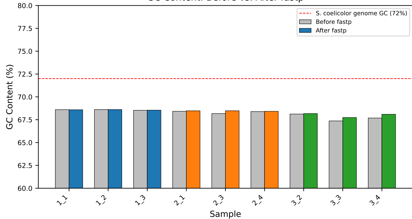
GC Content: Before vs. After fastp
