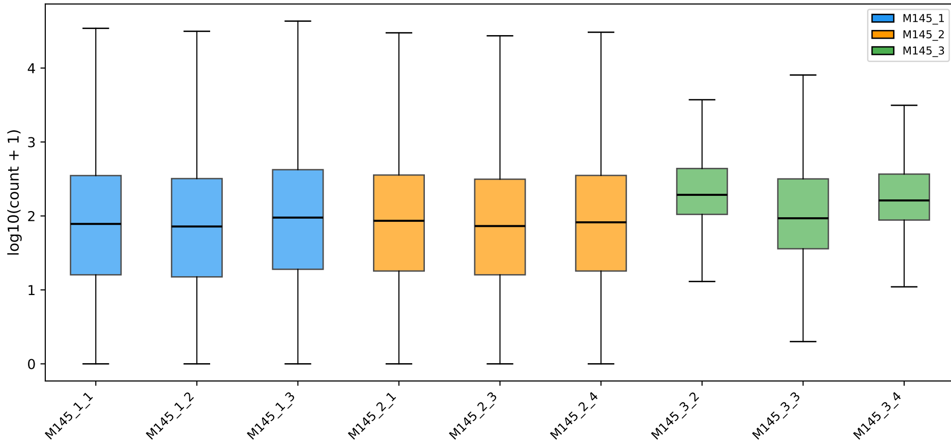
Gene Count Distribution per Sample
