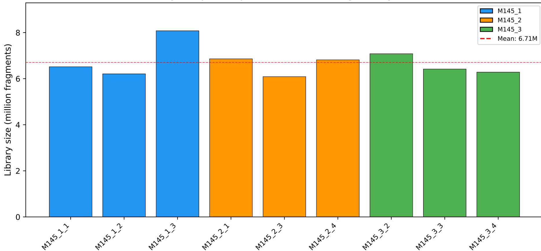
Library Size per Sample (featureCounts assigned fragments)
