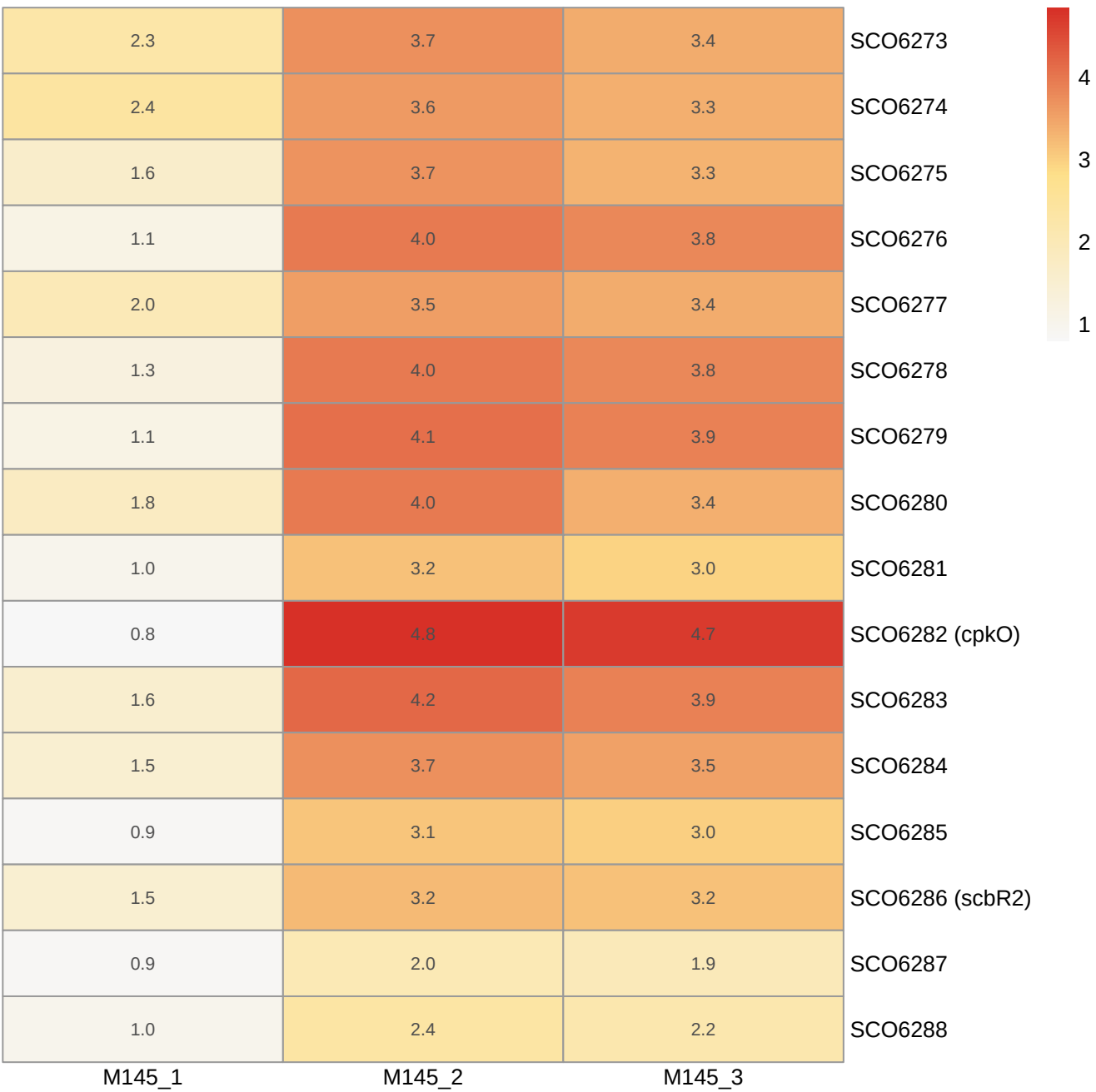
CPK cluster gene expression (log10)
