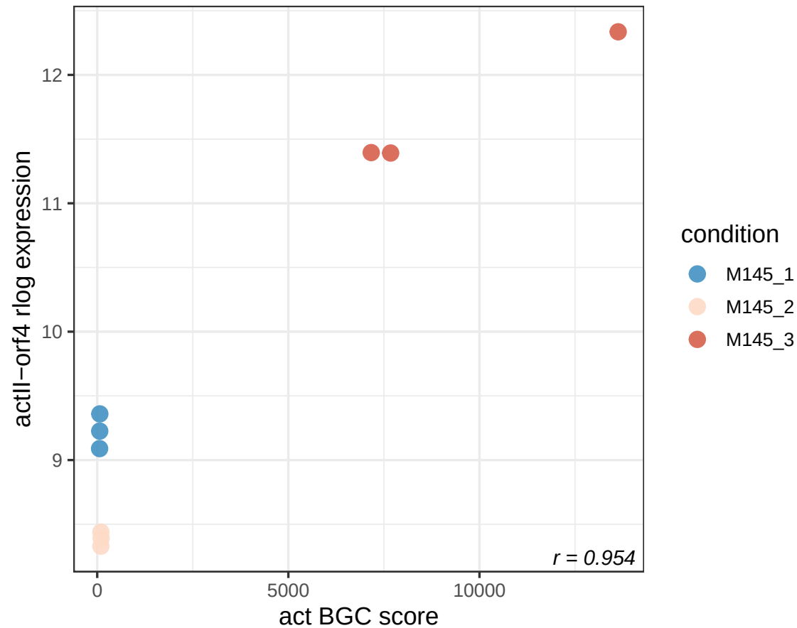
act score vs actII-orf4 (SC_RS27570)
