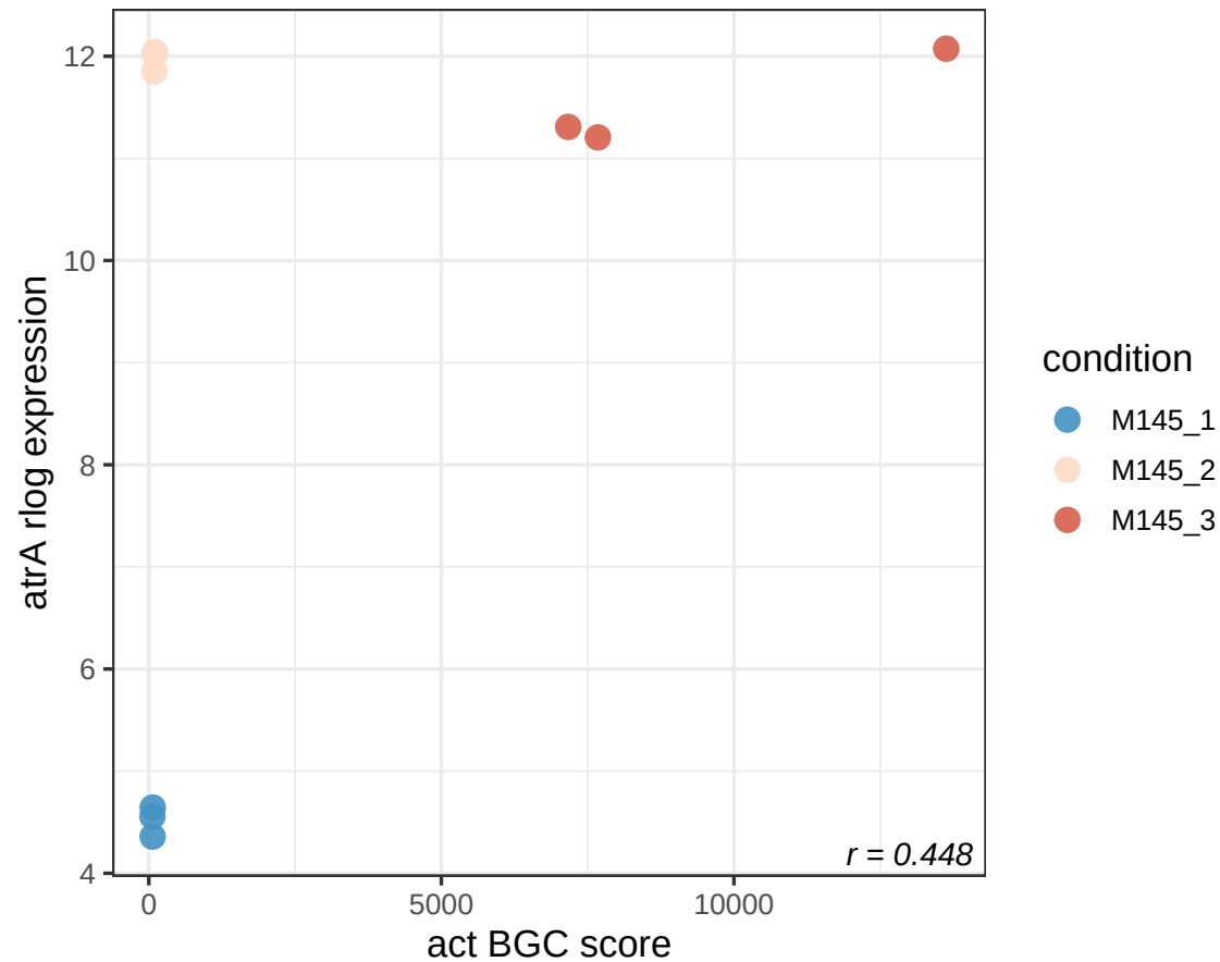
act score vs atrA (SC_RS25560)
