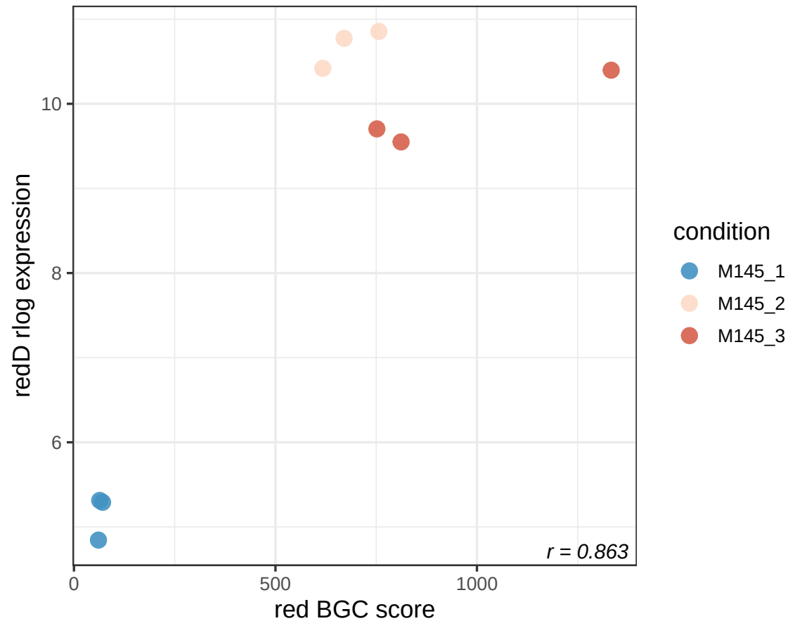
red score vs redD (SC_RS31630)
