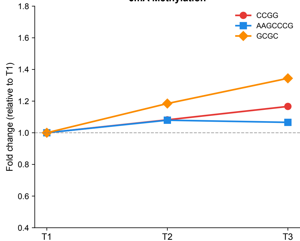
6mA Methylation
