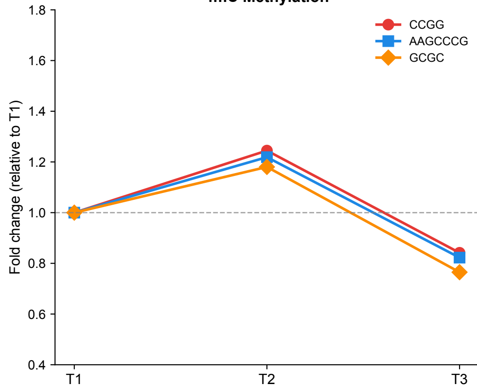
4mC Methylation
