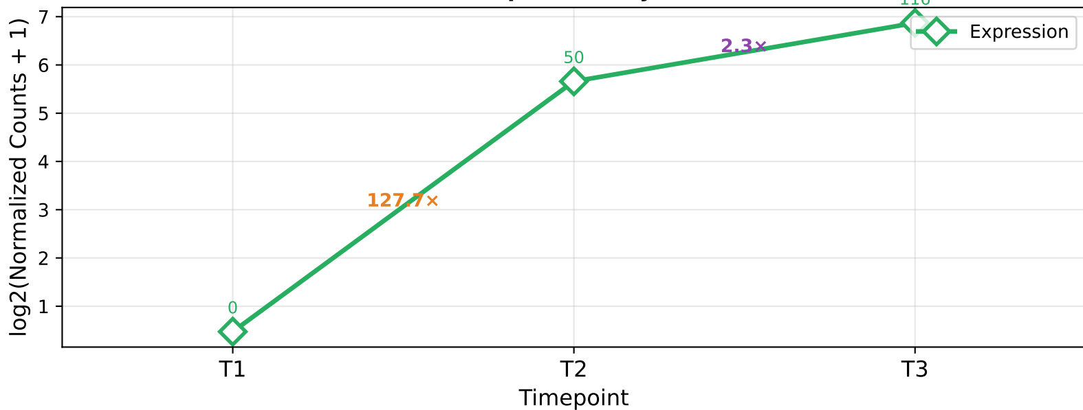
Gene Expression Dynamics
