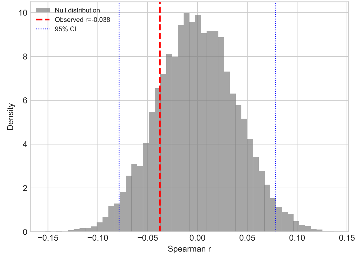
T3vsT1 6mA (n=662, perm p=0.0150)
