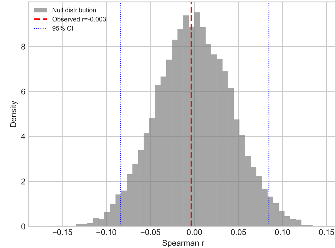
T3vsT1 4mC (n=542, perm p=0.9369)
