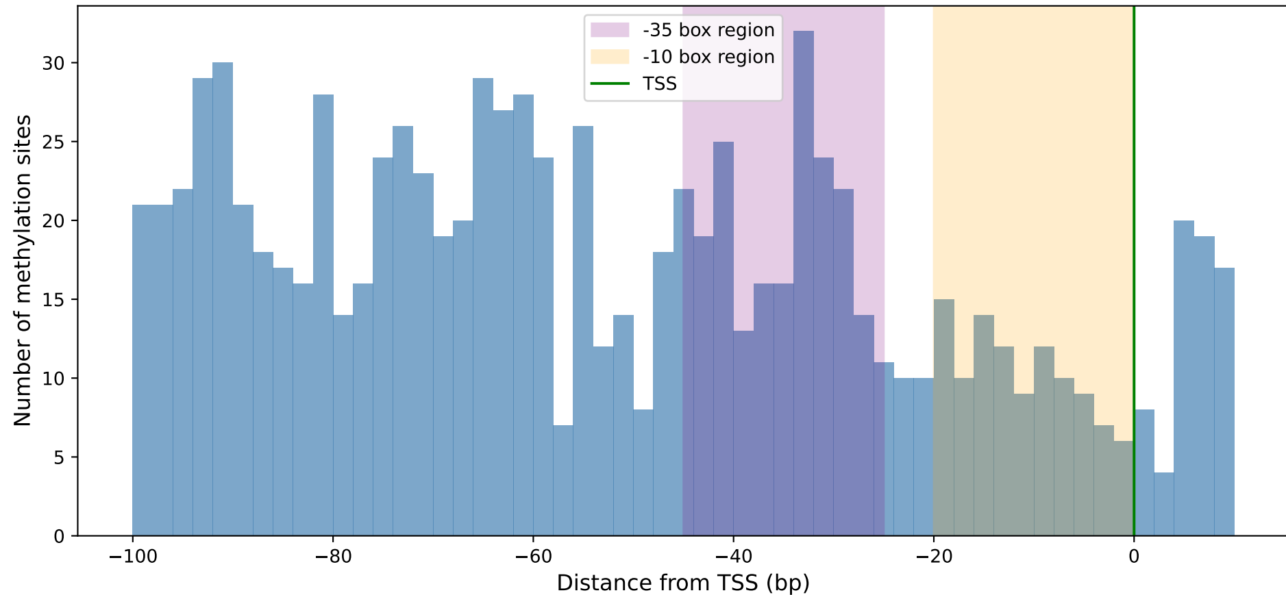
Methylation site distribution in core promoter region
