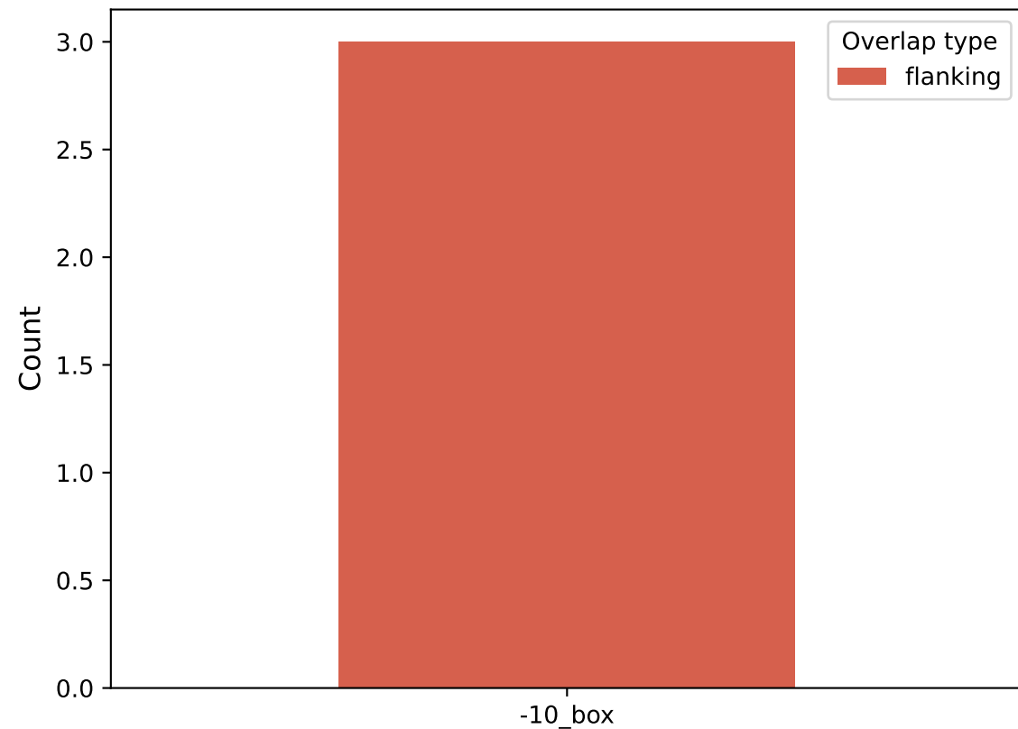
4mC at \sigma 70 motifs
