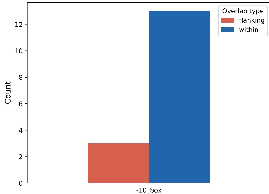
6mA at \sigma 70 motifs
