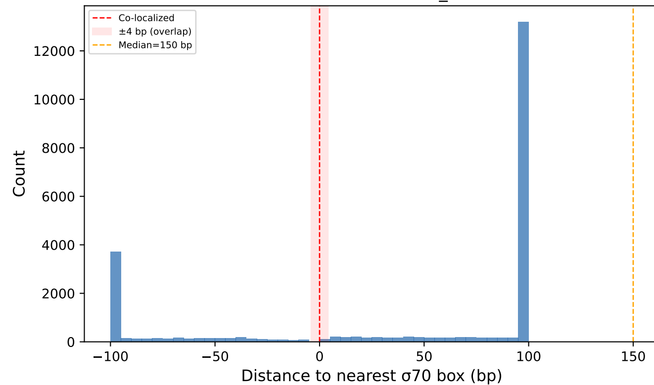
CCGG \rightarrow nearest -10_box
