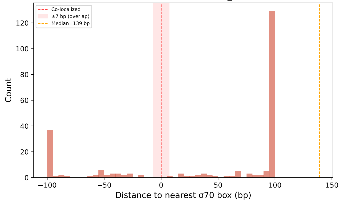
AAGCCCG \rightarrow nearest -10_box
