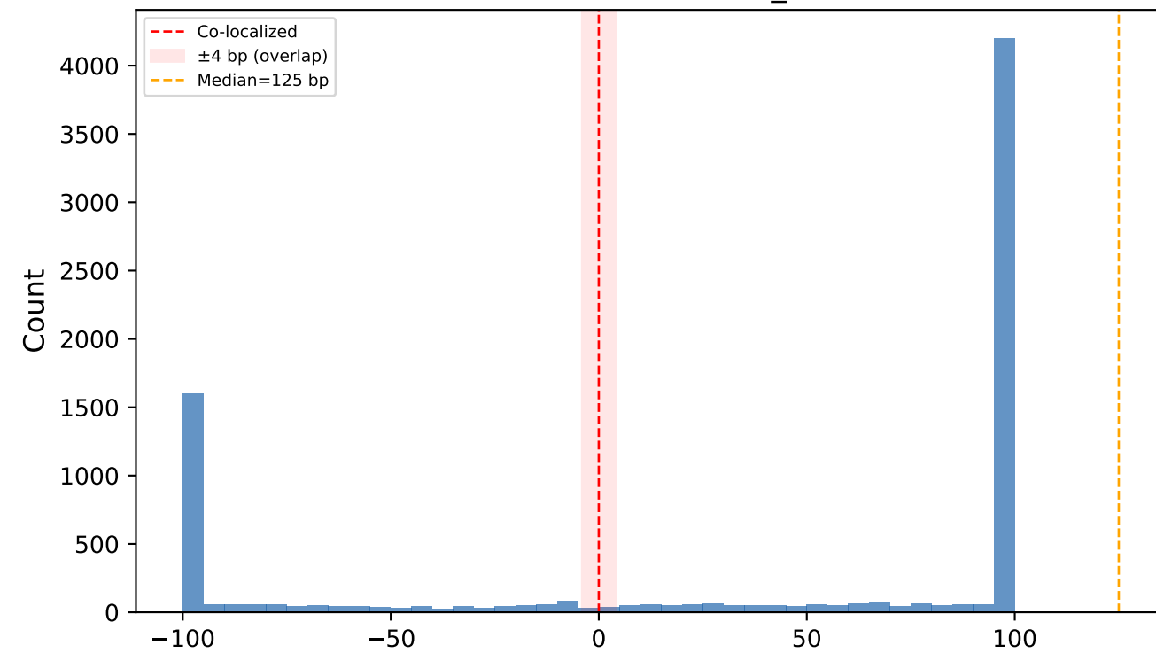
CCGG \rightarrow nearest -10_box
