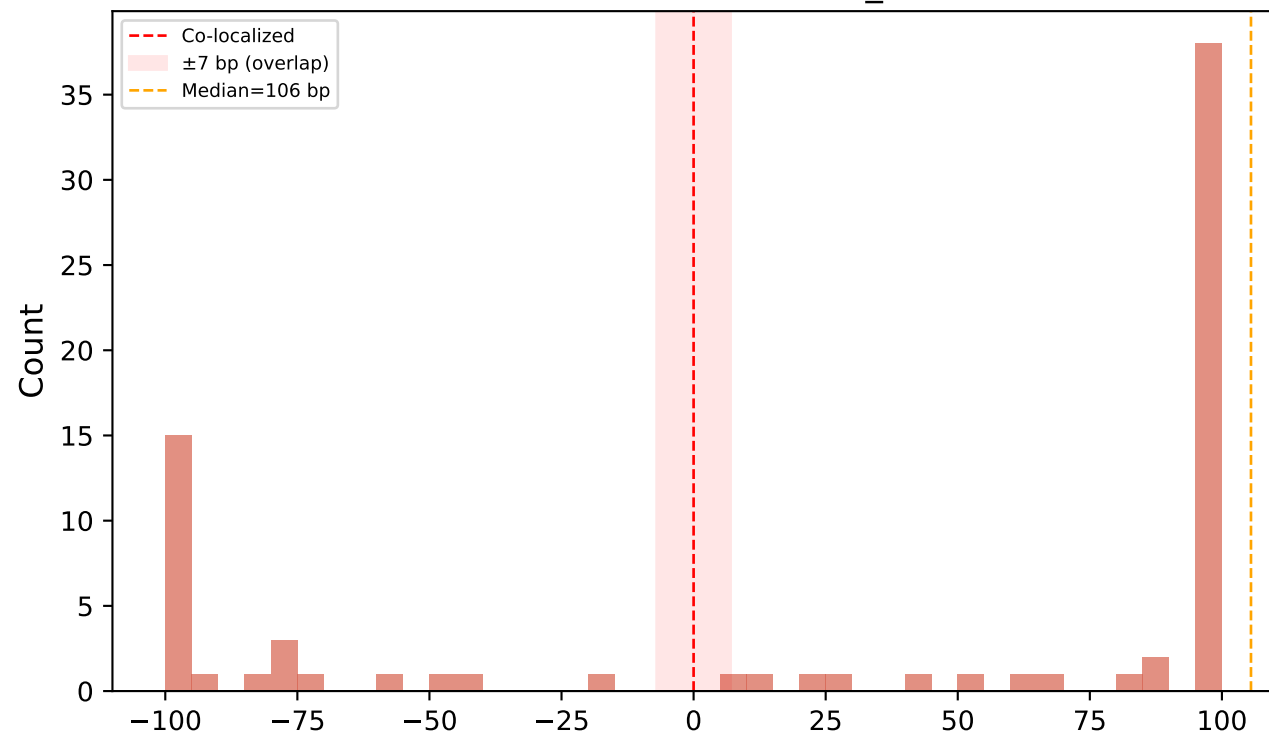
AAGCCCG \rightarrow nearest -10_box
