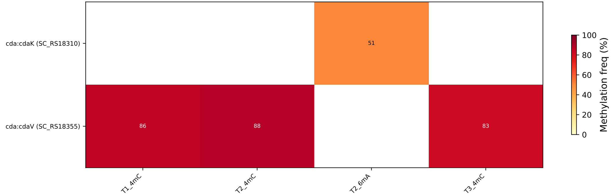
BGC gene SARP zone methylation (freq %)
