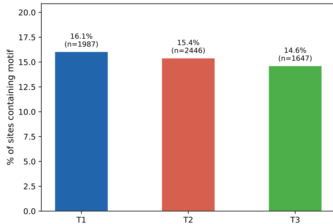
4mC — GCGC
