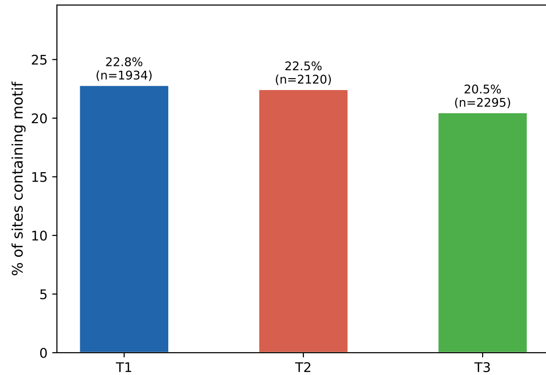
4mC — GCGC
