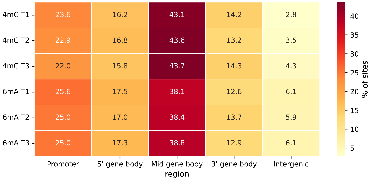
Genomic Region Distribution (%) by Modification Type and Timepoint
