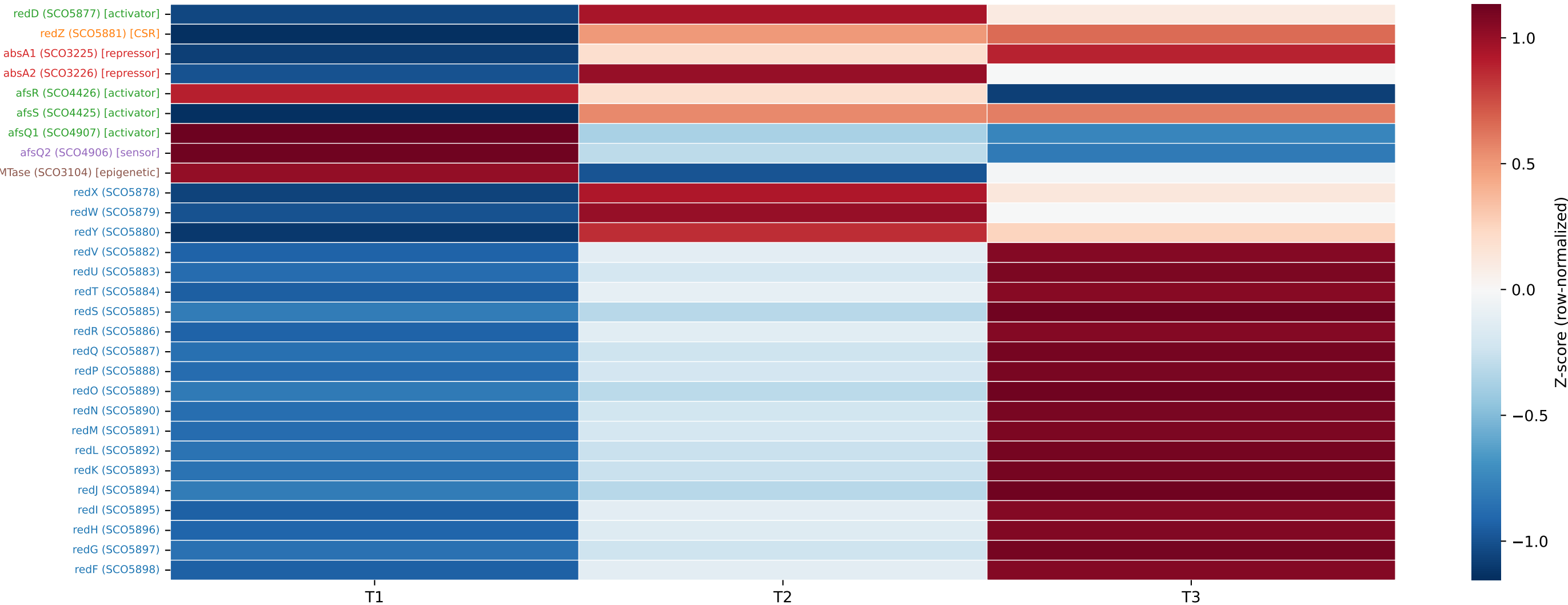
C. Expression Heatmap: Red BGC Regulators & Structural Genes
