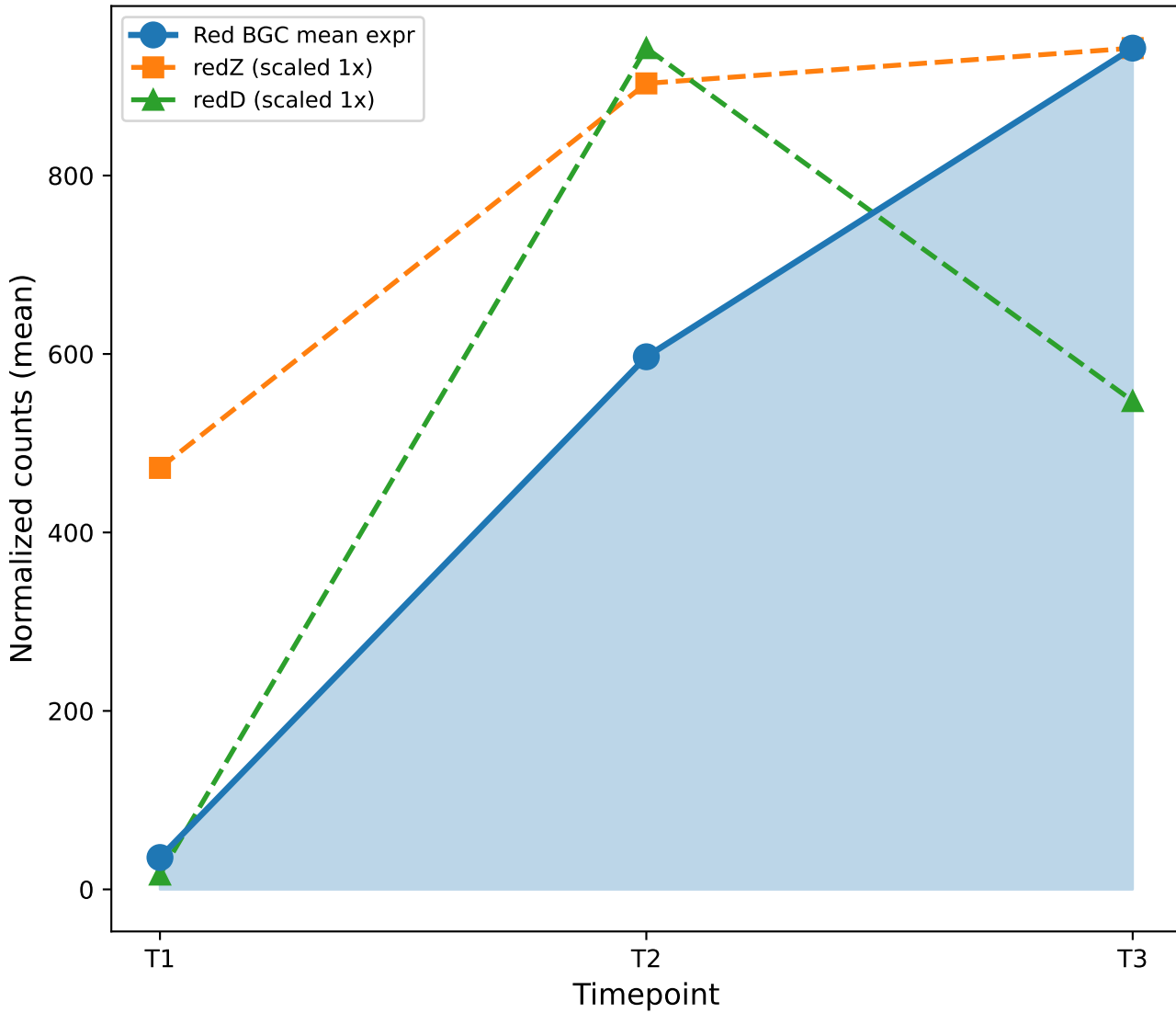
B. Red BGC Expression vs Key Regulators
