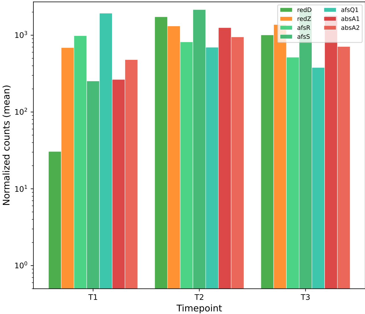
A. Regulator Expression Timeline
