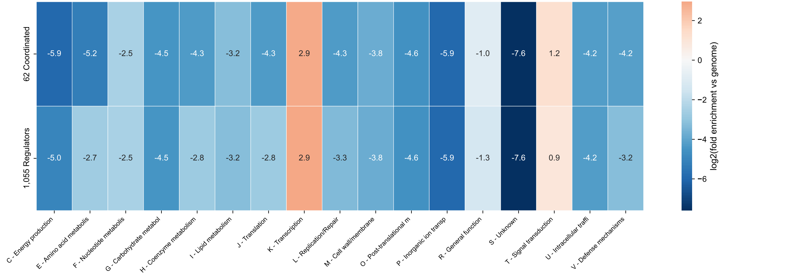
B. log2 fold enrichment vs genome-wide background
