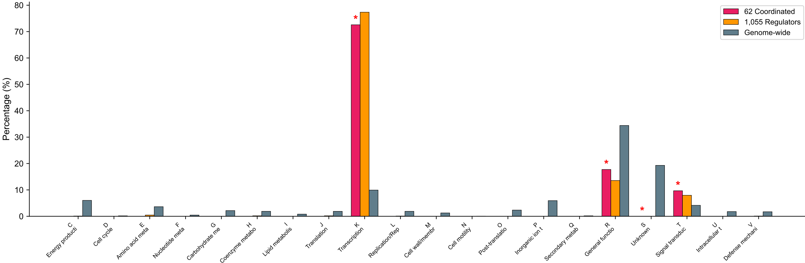
A. COG category distribution: 62 coordinated vs 1,055 regulators vs genome
