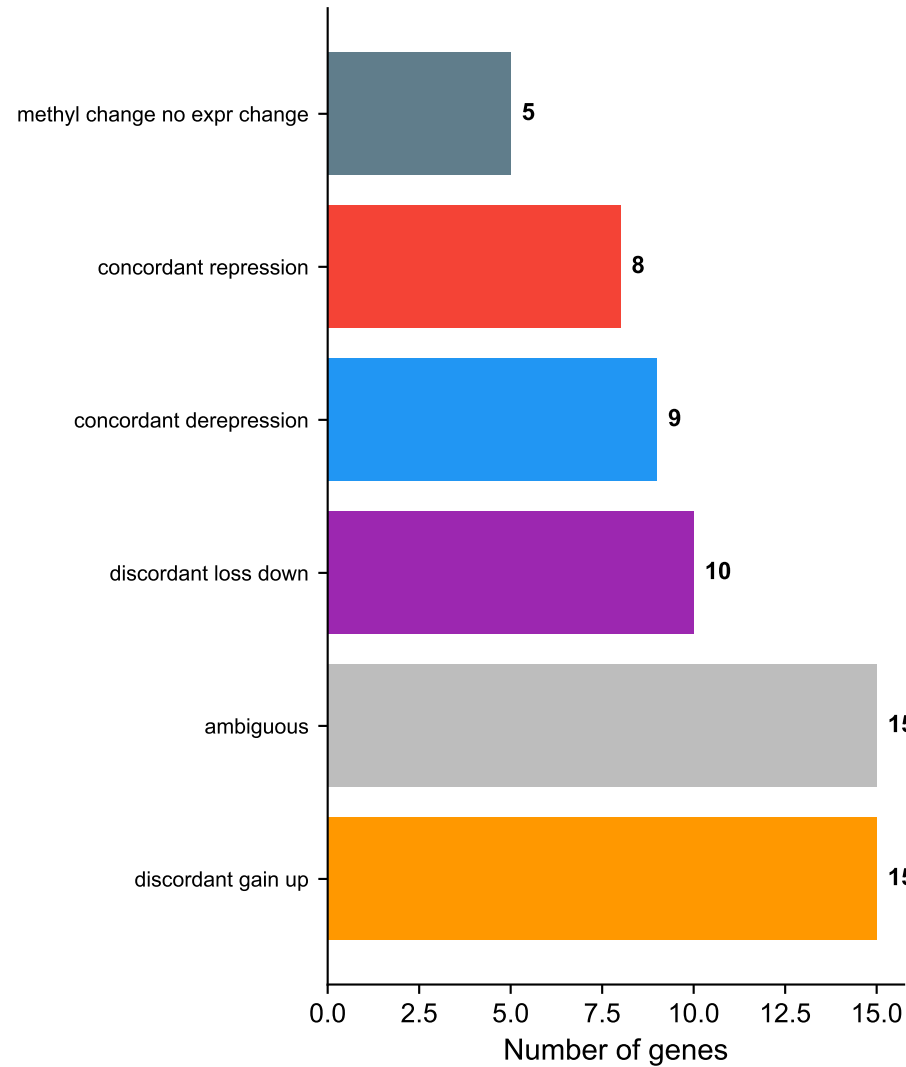
B. T3 coordination types
