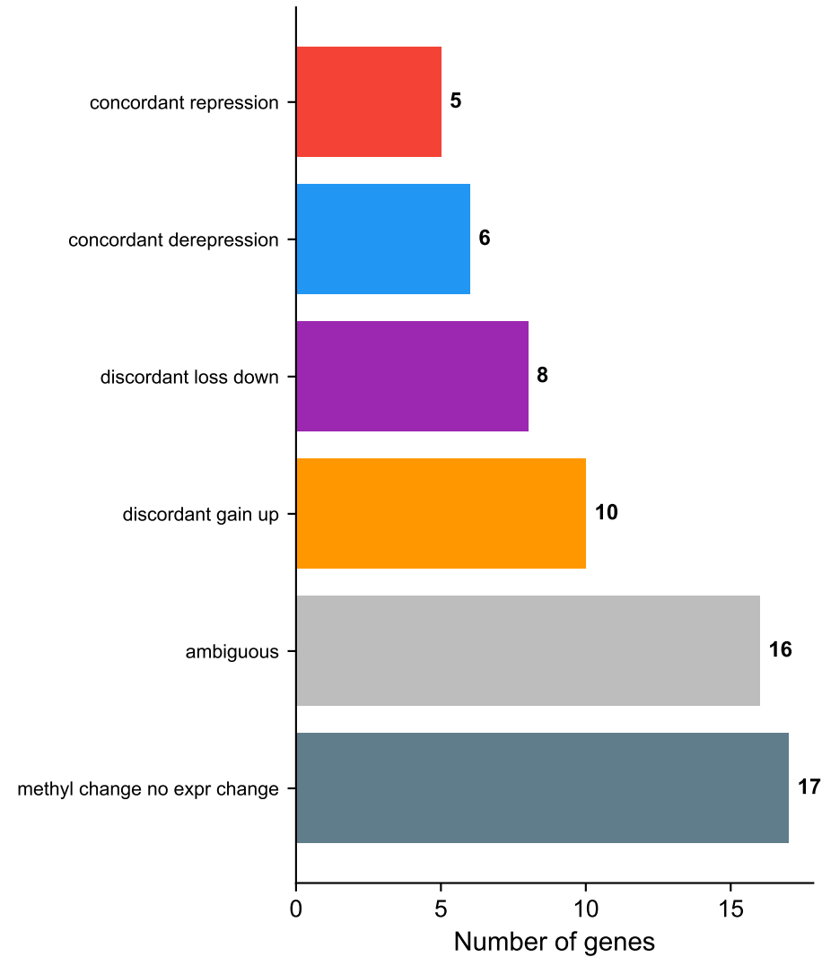
A. T2 coordination types
