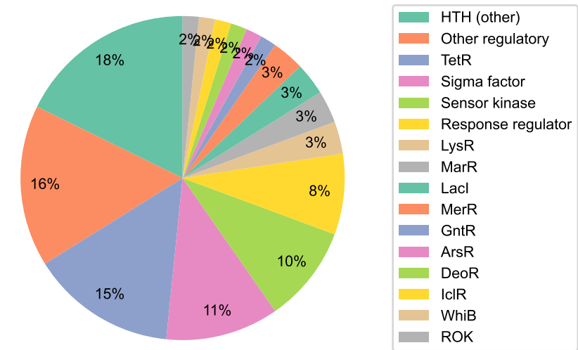
C. TF family distribution
