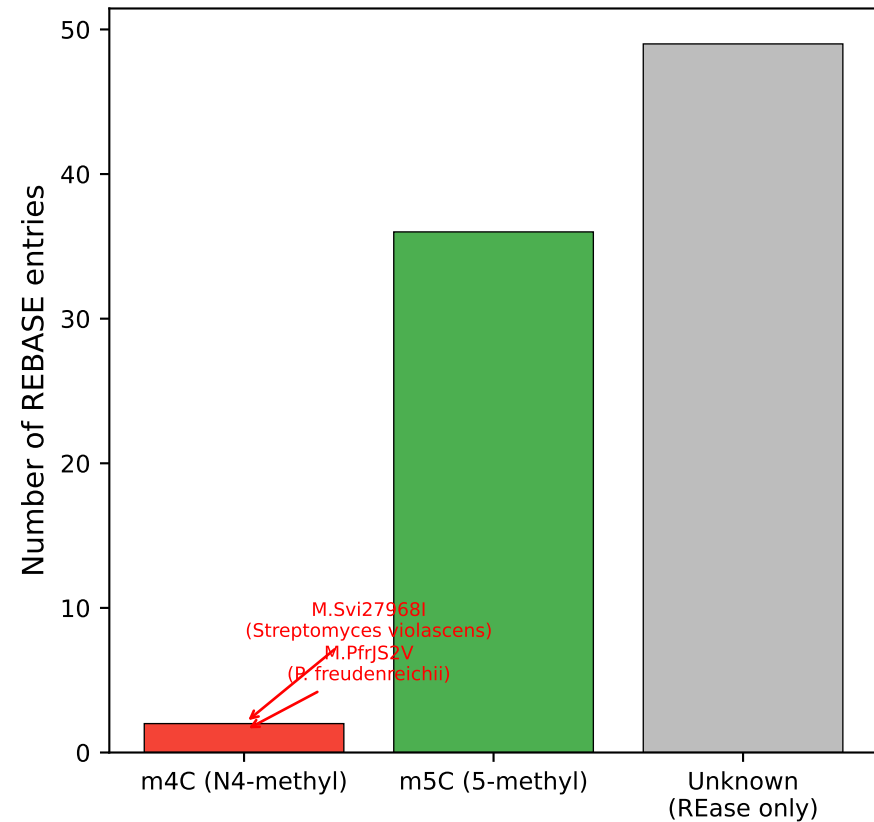
C. GCCGGC methylation specificity (known MTases)
