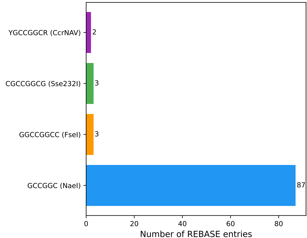
A. GCCGGC-containing recognition sequences
