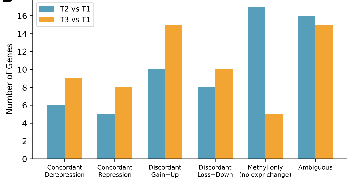
D Coordination Types in 62 Regulators
