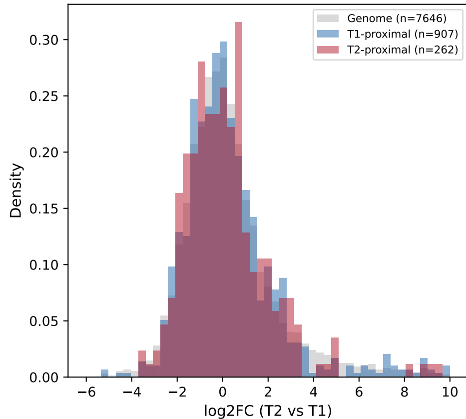
Expression change (AAGCCCG-proximal vs genome)
