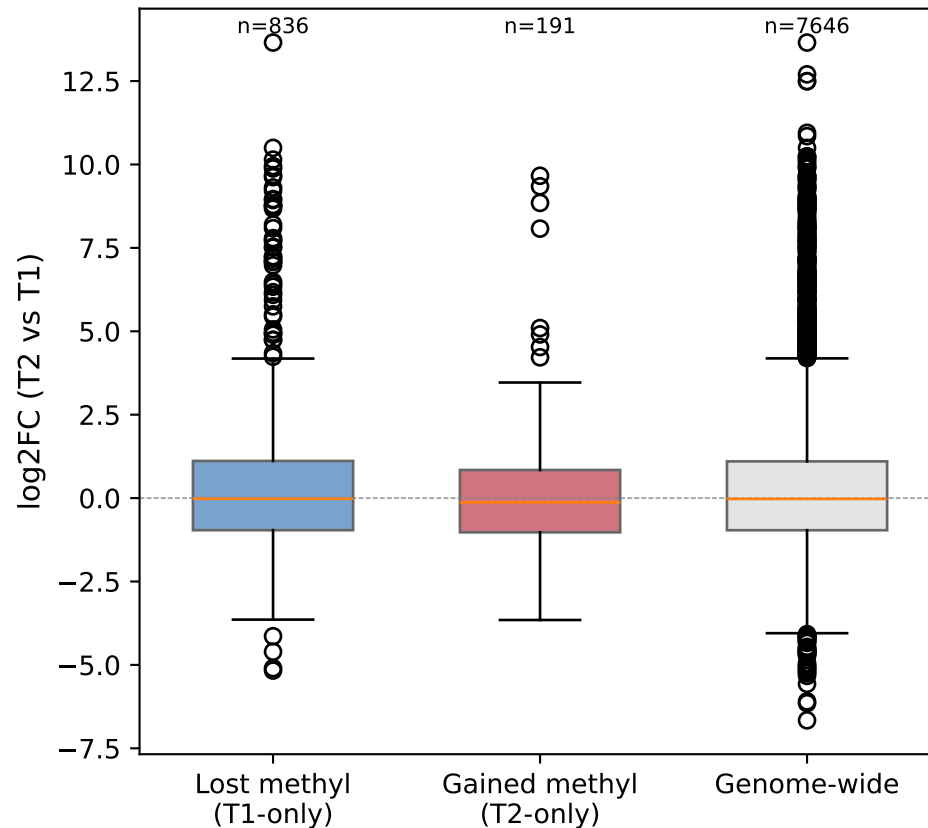
Expression by methylation change
