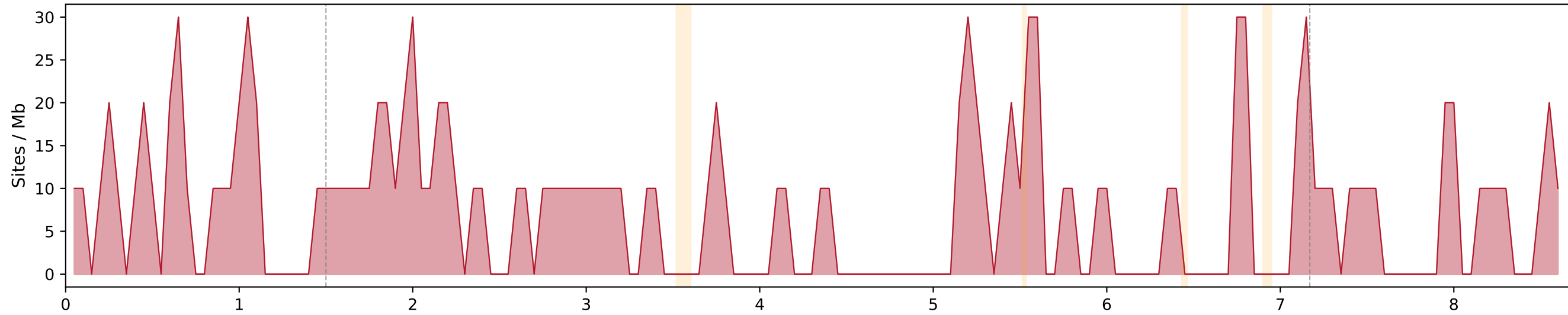
T2: AAGCCCG sites (n=64)
