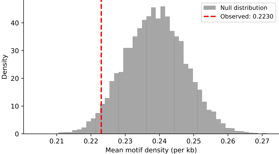
E. Permutation Test: TGGCCGGC Extended Region
