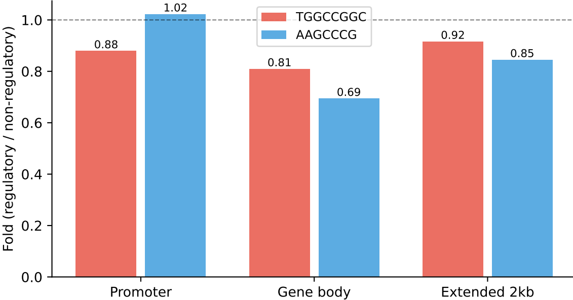
B. DNA Motif Density Fold by Gene Zone
