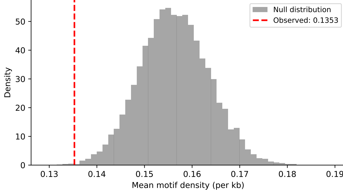
F. Permutation Test: AAGCCCG Extended Region
