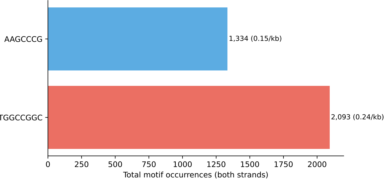
A. Genome-wide Motif Counts
