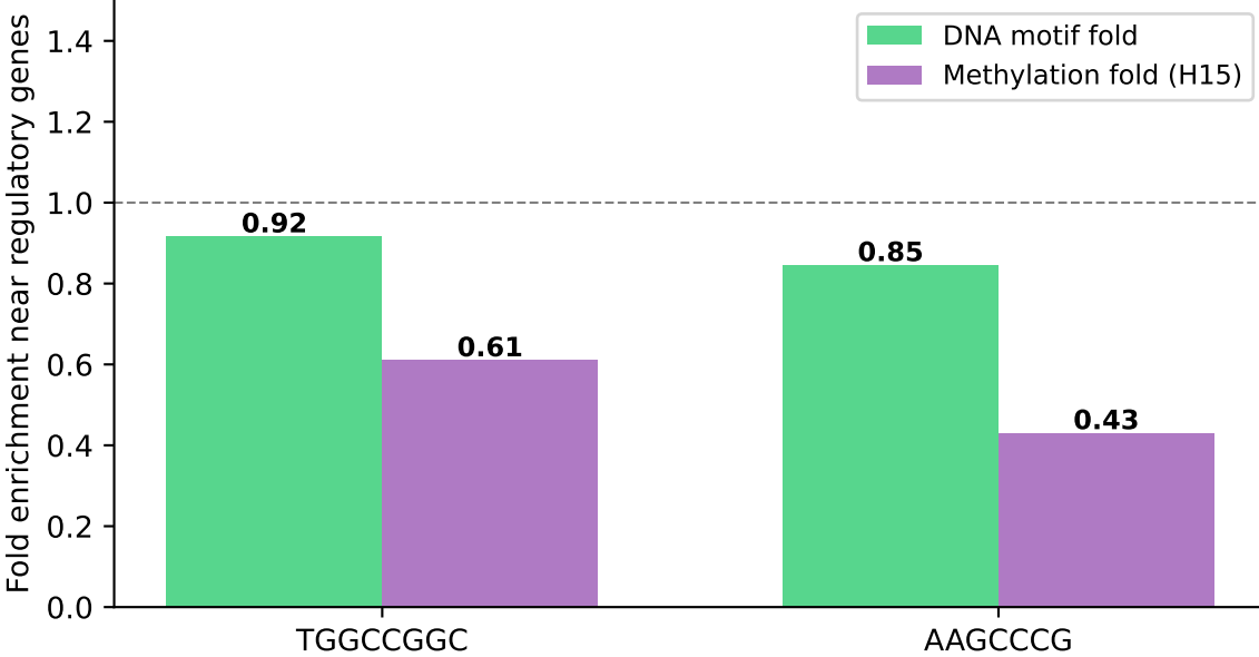
D. Sequence vs Methylation Depletion
