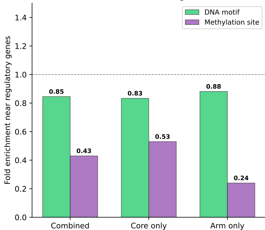
AAGCCCG (6mA recognition)
