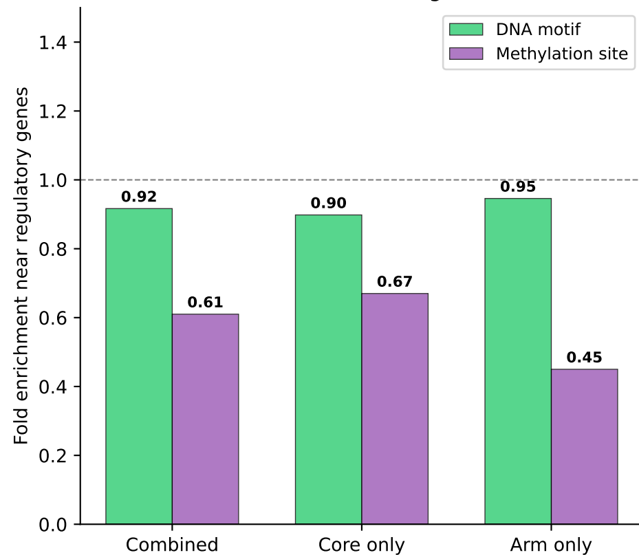
CCCGGC (4mC recognition)
