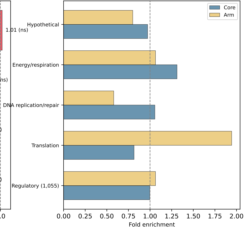
E. Core vs Arm (GCCGGC)
