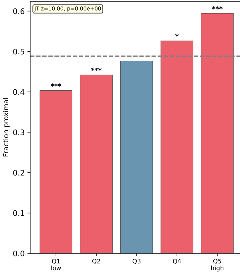
C. Expression Quintile (GCCGGC)
