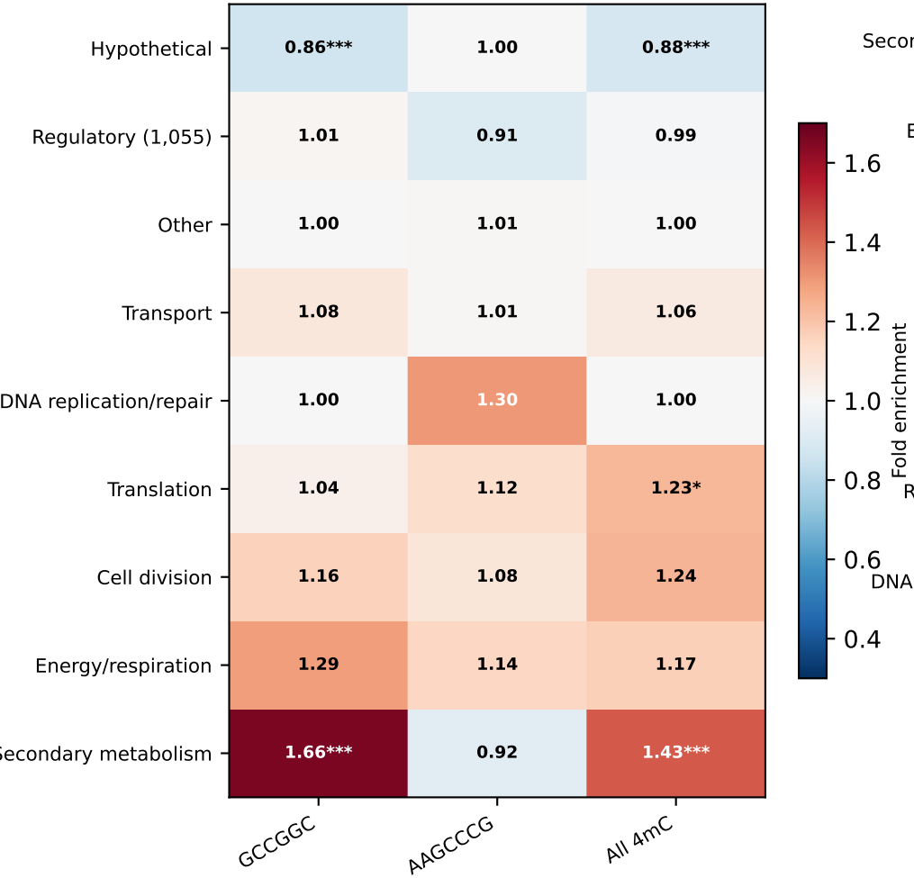
A. Category × Motif Heatmap
