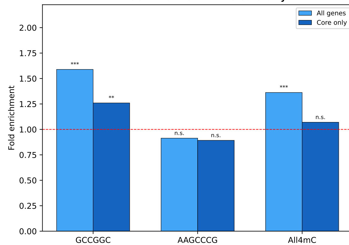
B. BGC Enrichment: All vs Core-only
