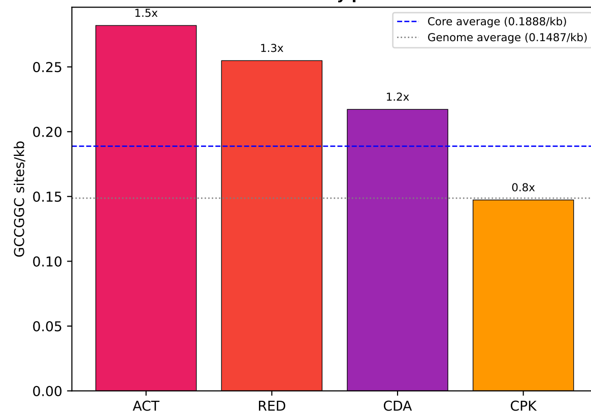
D. GCCGGC Density per BGC Cluster
