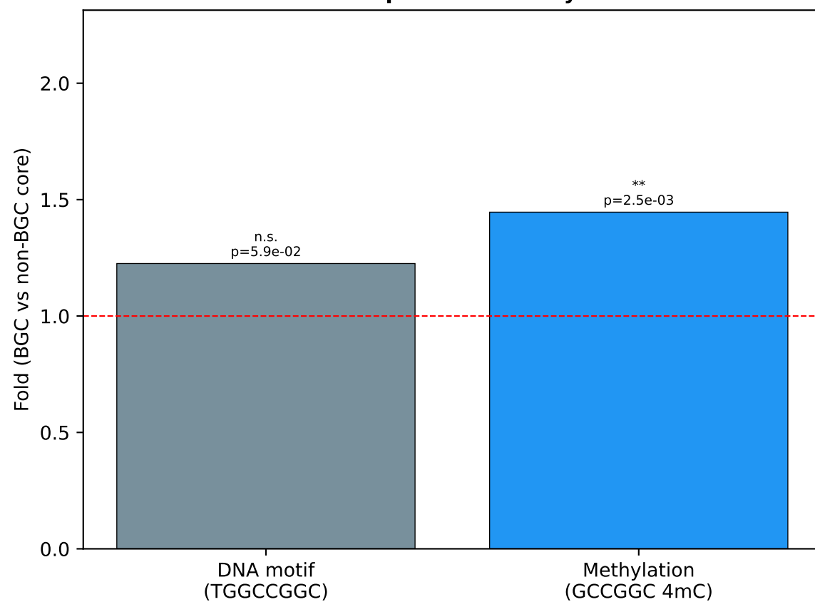
C. DNA Sequence vs Methylation
