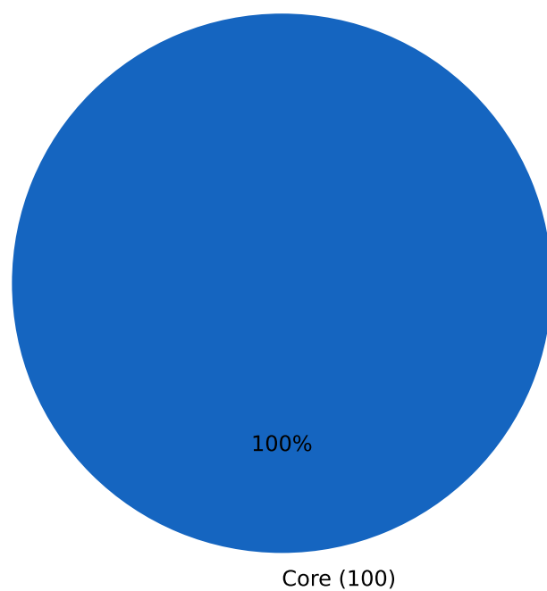
A. BGC Gene Geography
