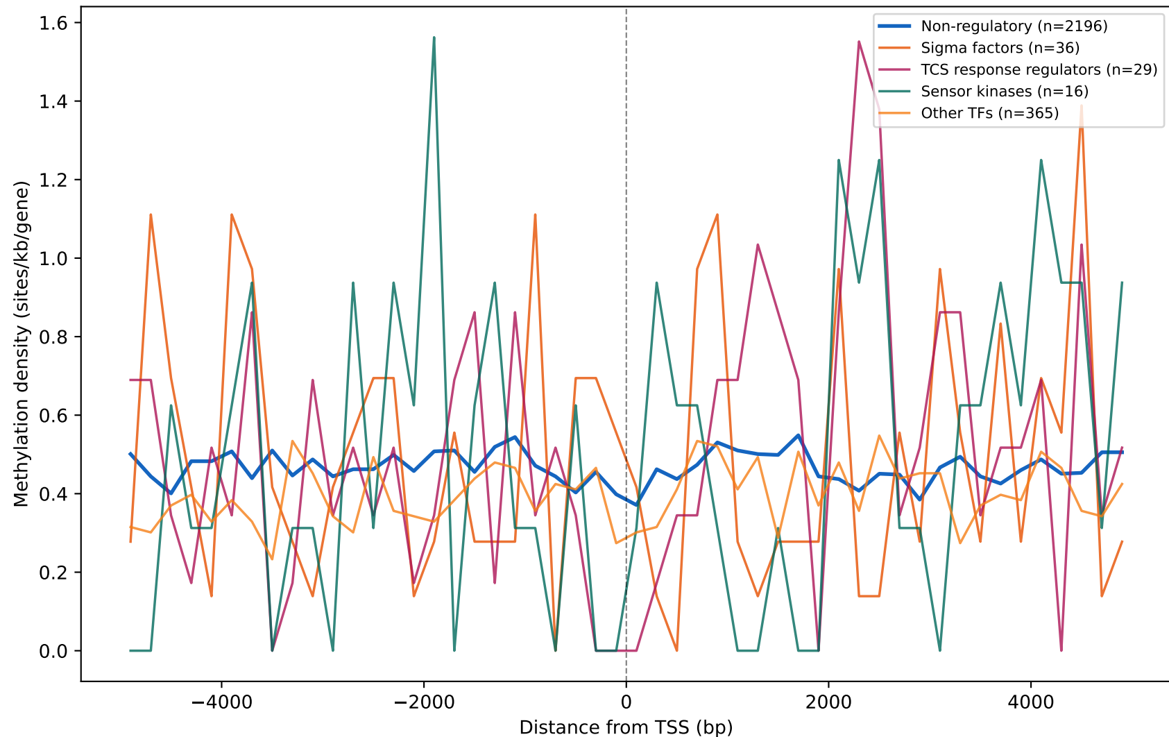
Regulatory sub-type methylation profiles (All sites, T1)
